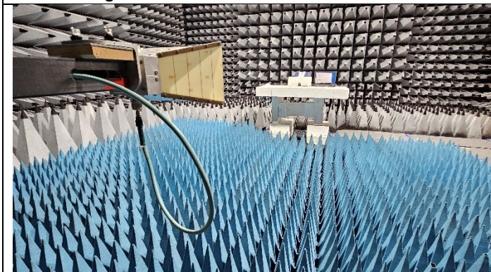
Fig A5: Radiated Emissions Above 1GHz
