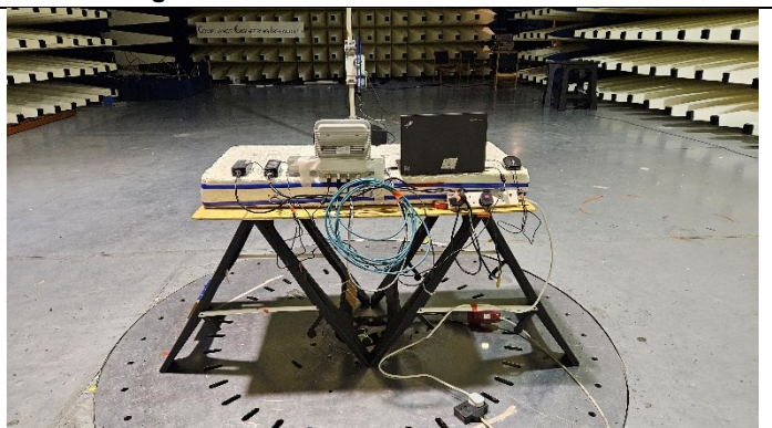
Fig A4: Radiated Emissions Below 1GHz
