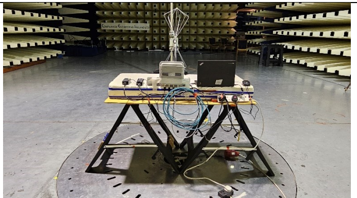
Fig A2: Radiated Emissions Below 1GHz
