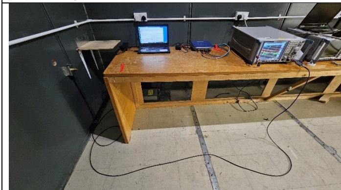
Fig A7: Conducted Emission on Mains
