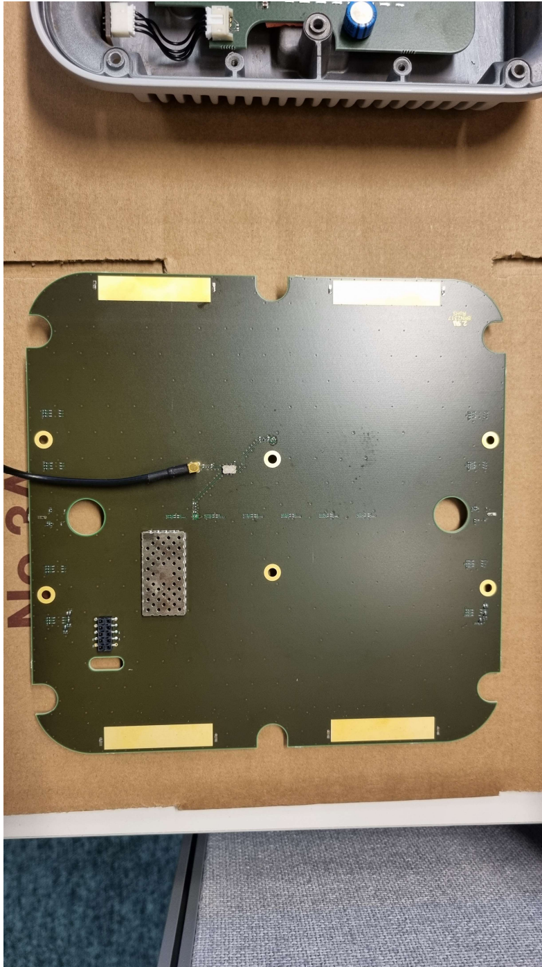
Picture 6. IRX200 RFID antenna radiator bottom side.
