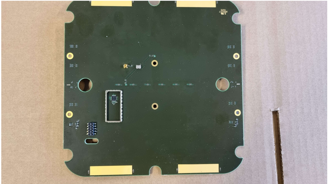
Picture 7. IRX200 RFID antenna radiator bottom side without RF shield.
