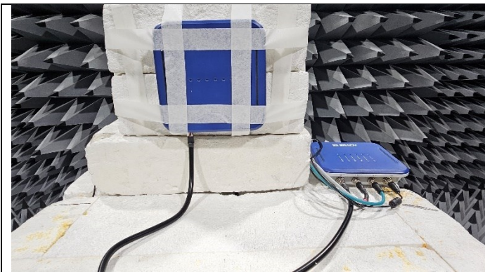
Fig G4: EUT Orientation "O1" External Antenna
