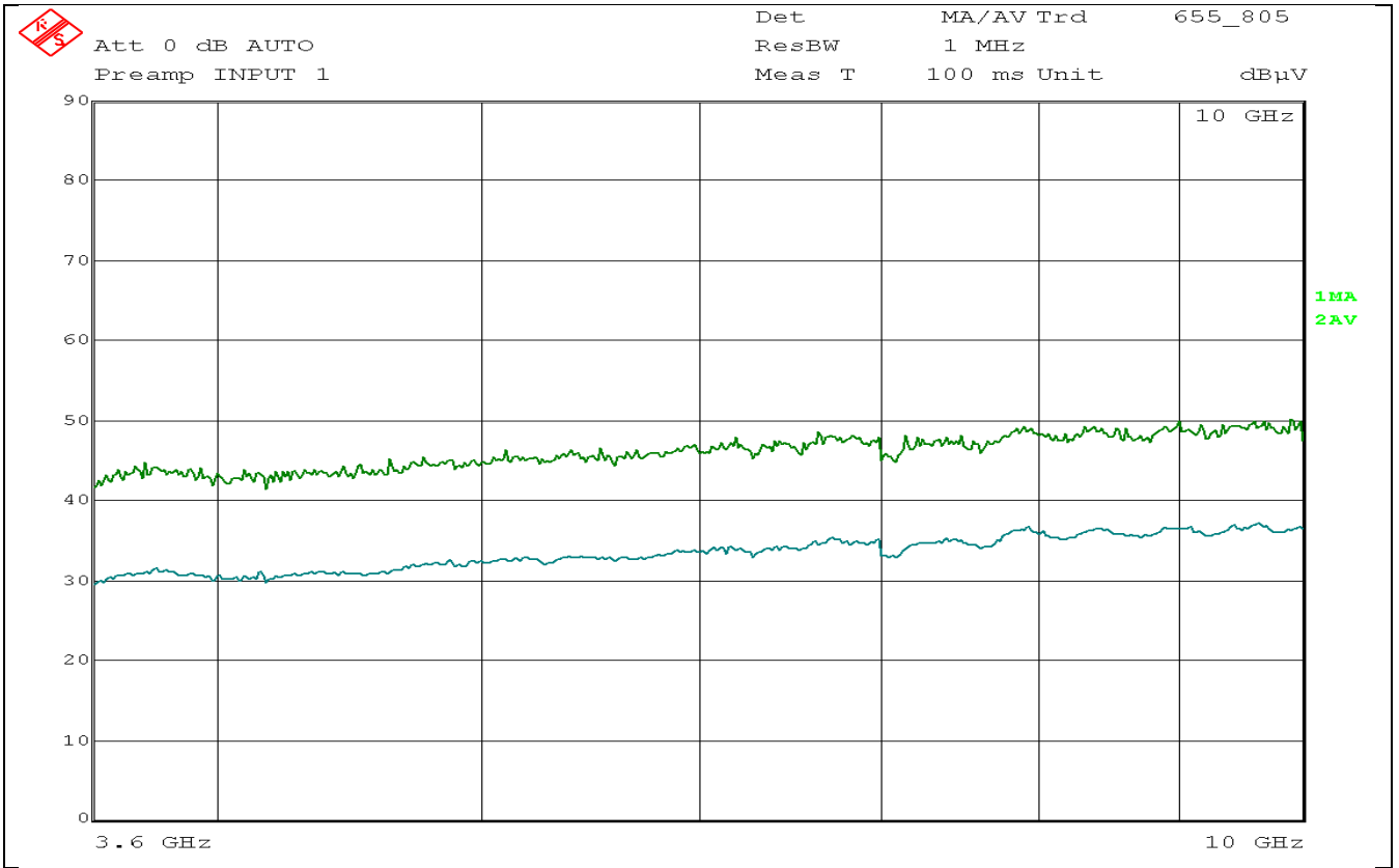
Fig D7: Low Channel Radiated Emissions 3.6GHz - 10GHz, Vertical, 3metre
