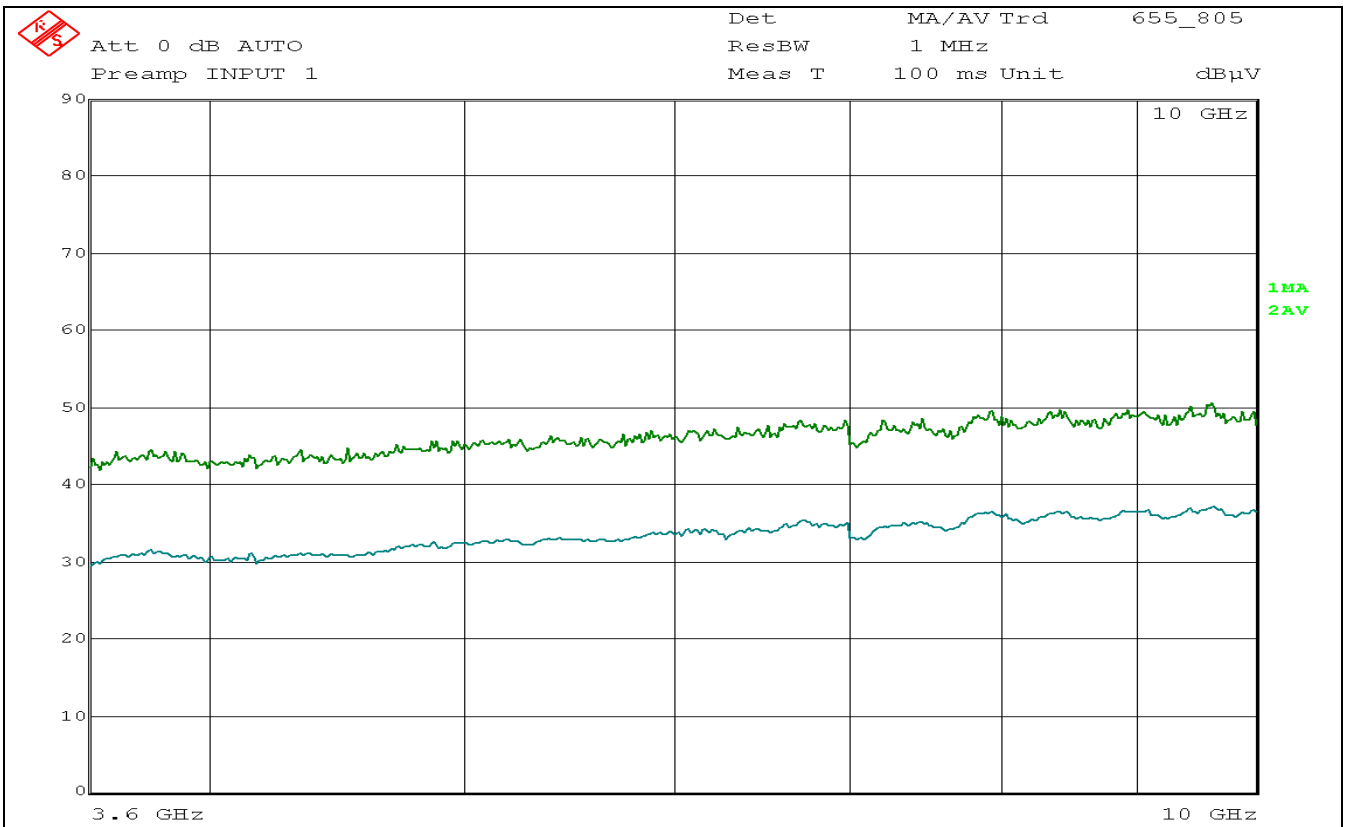
Fig D8: Low Channel Radiated Emissions 3.6GHz - 10GHz, Horizontal, 3metre
