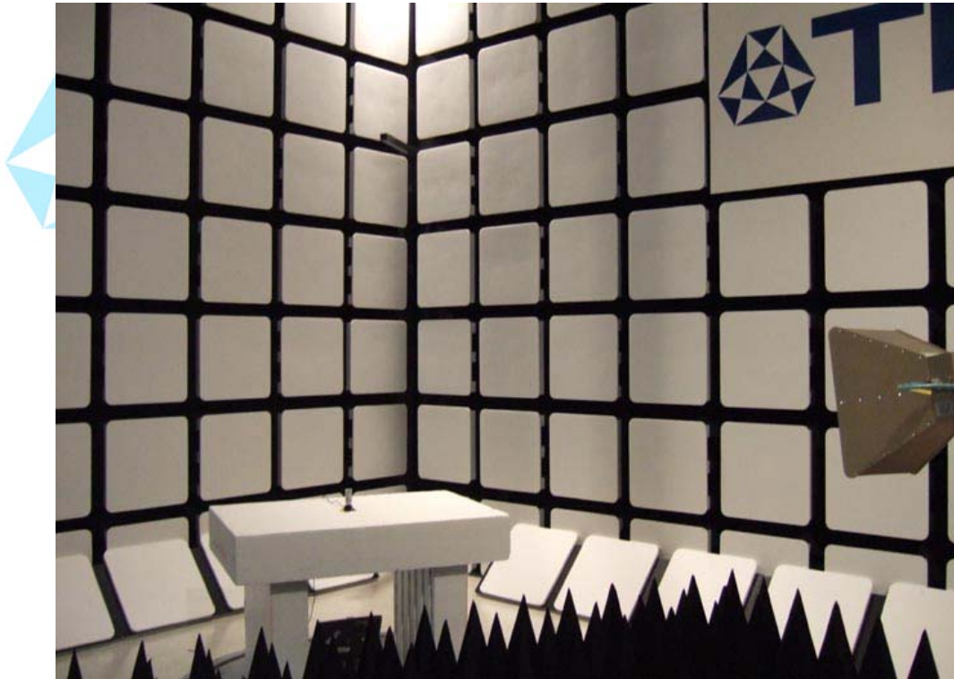
Test Configuration 3: 960 MHz to 40 GHz
