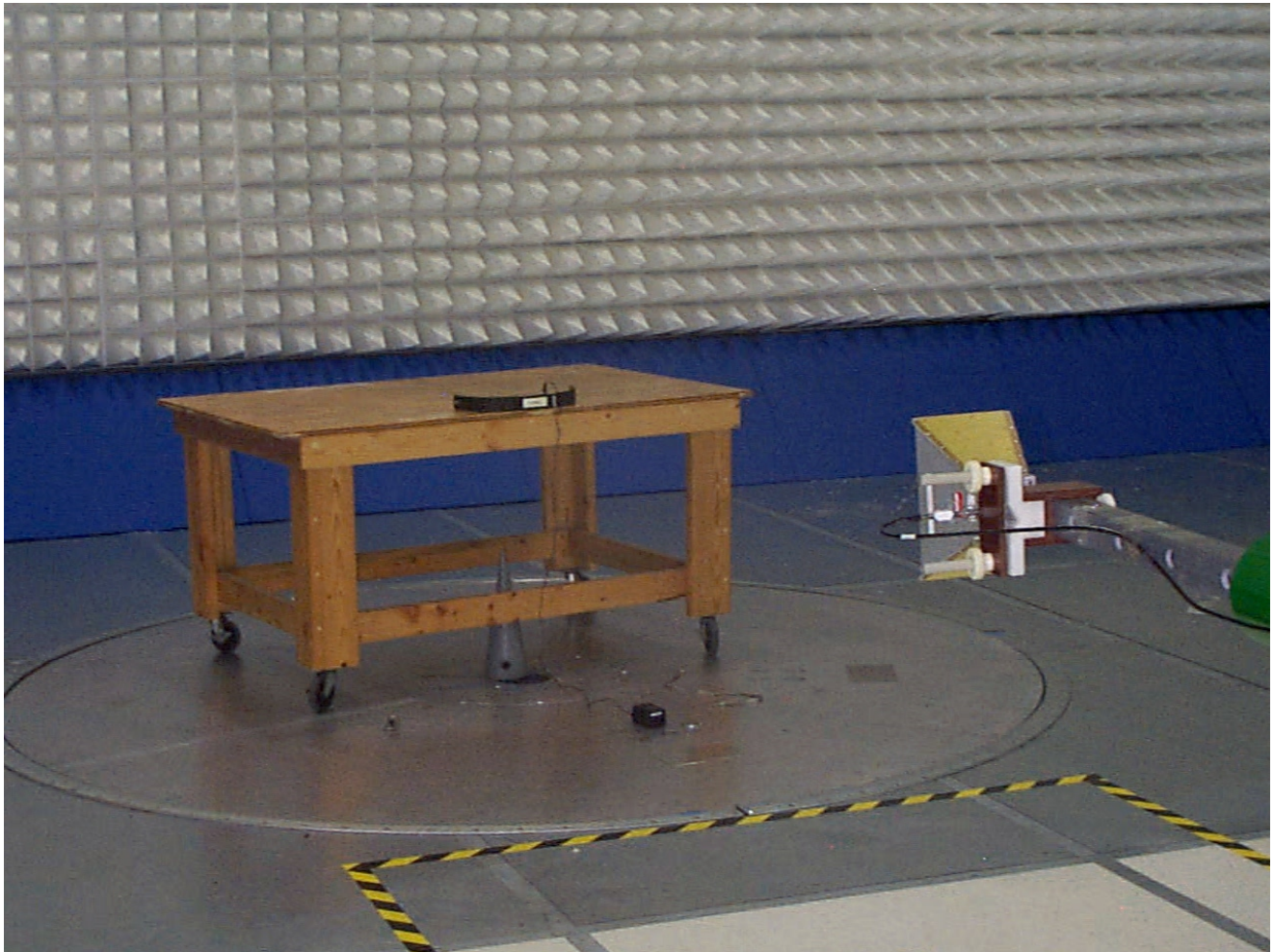
Figure 4: Radiated Testing 2
