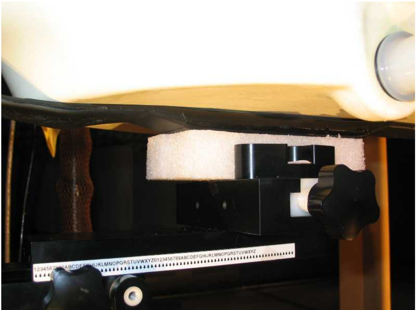
Figure 1: SAR Testing
