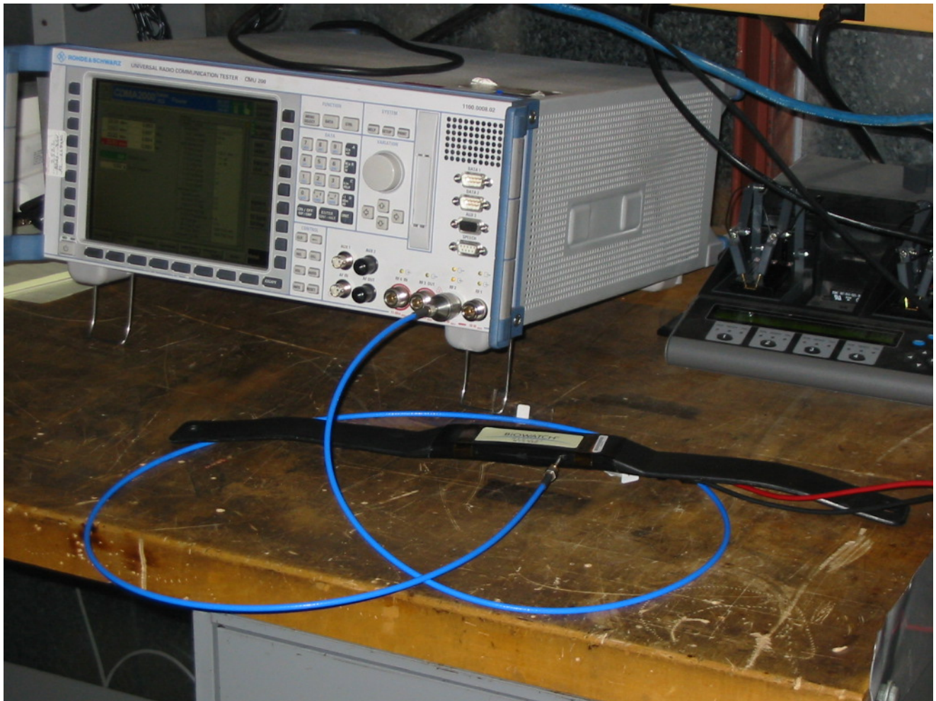
Figure 2: Conducted Testing
