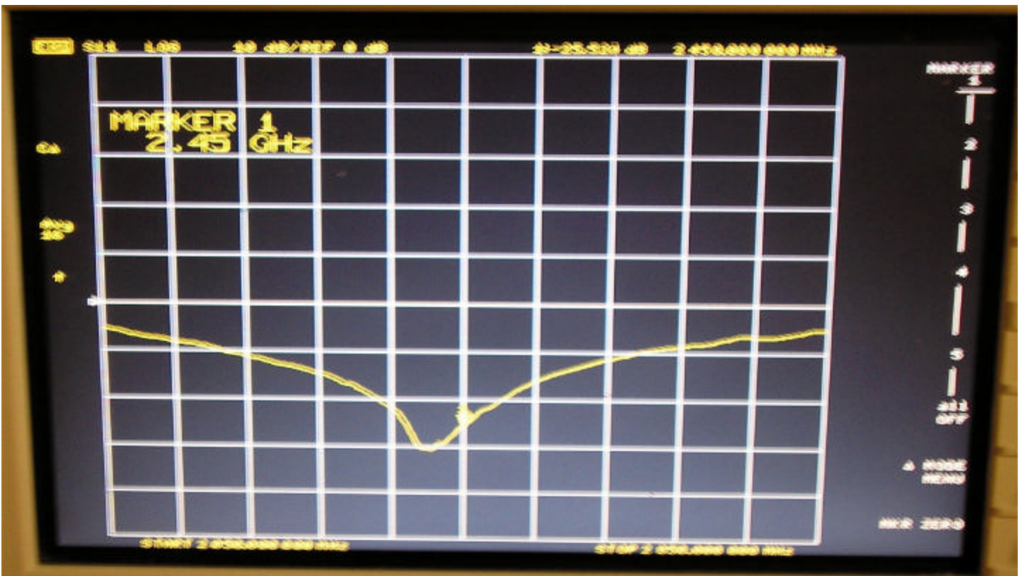
2450 dipole verification return loss data 8/20/2004
