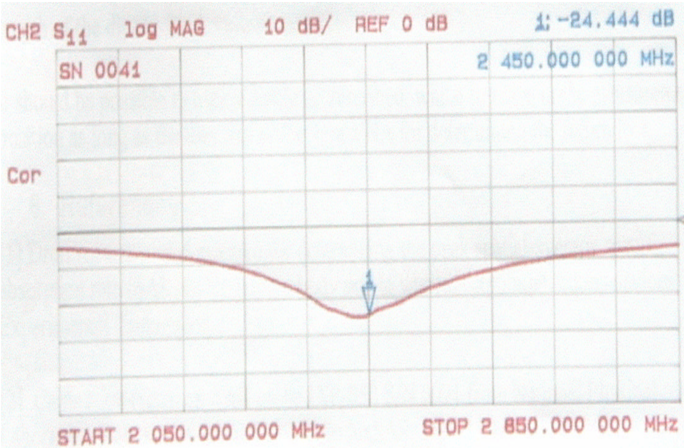
2450MHz dipole MFR return loss data.
