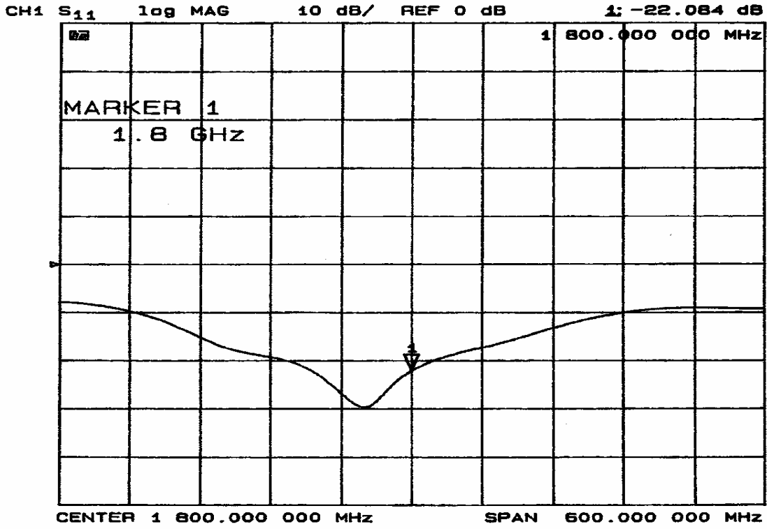
1800MHz Dipole MFR return loss Data
