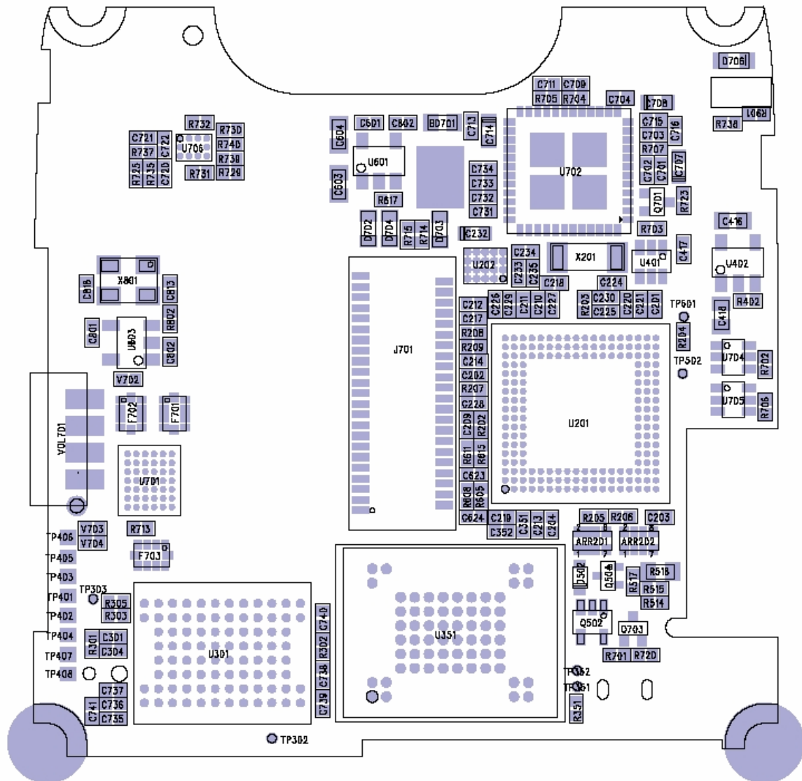
<Figure 5.1> Top View
