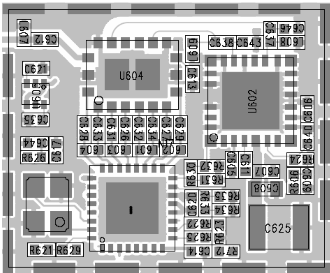
<Figure 5.3> RF Area
