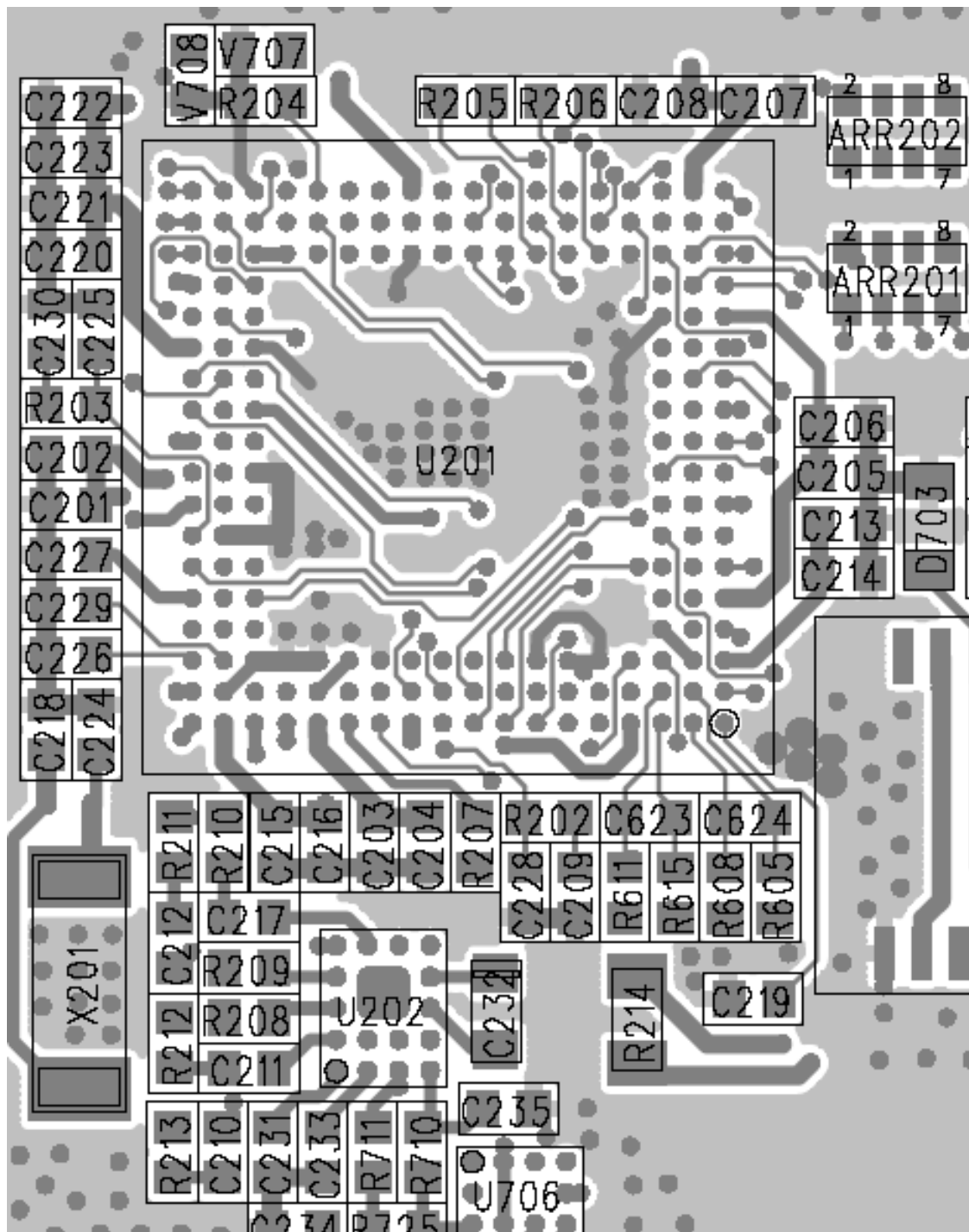
<Figure 5.5> BASEBAND Area
