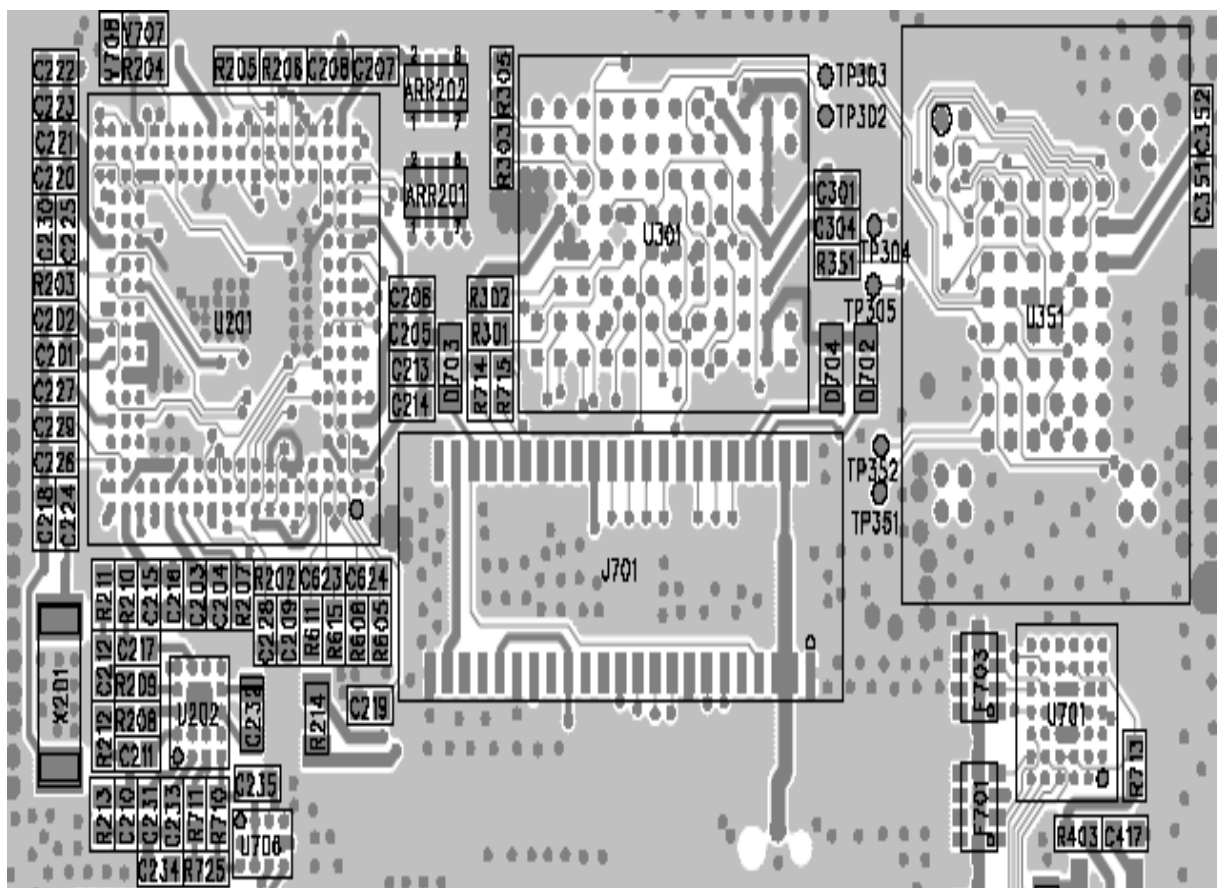
<Figure 5.3> Module Area
