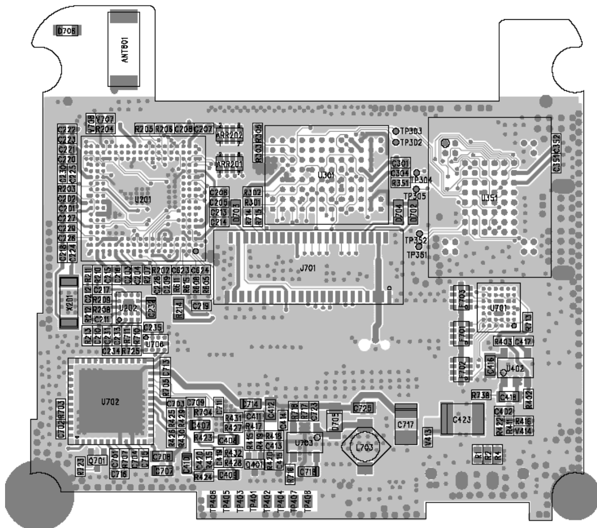
<Figure 5.1> Top View
