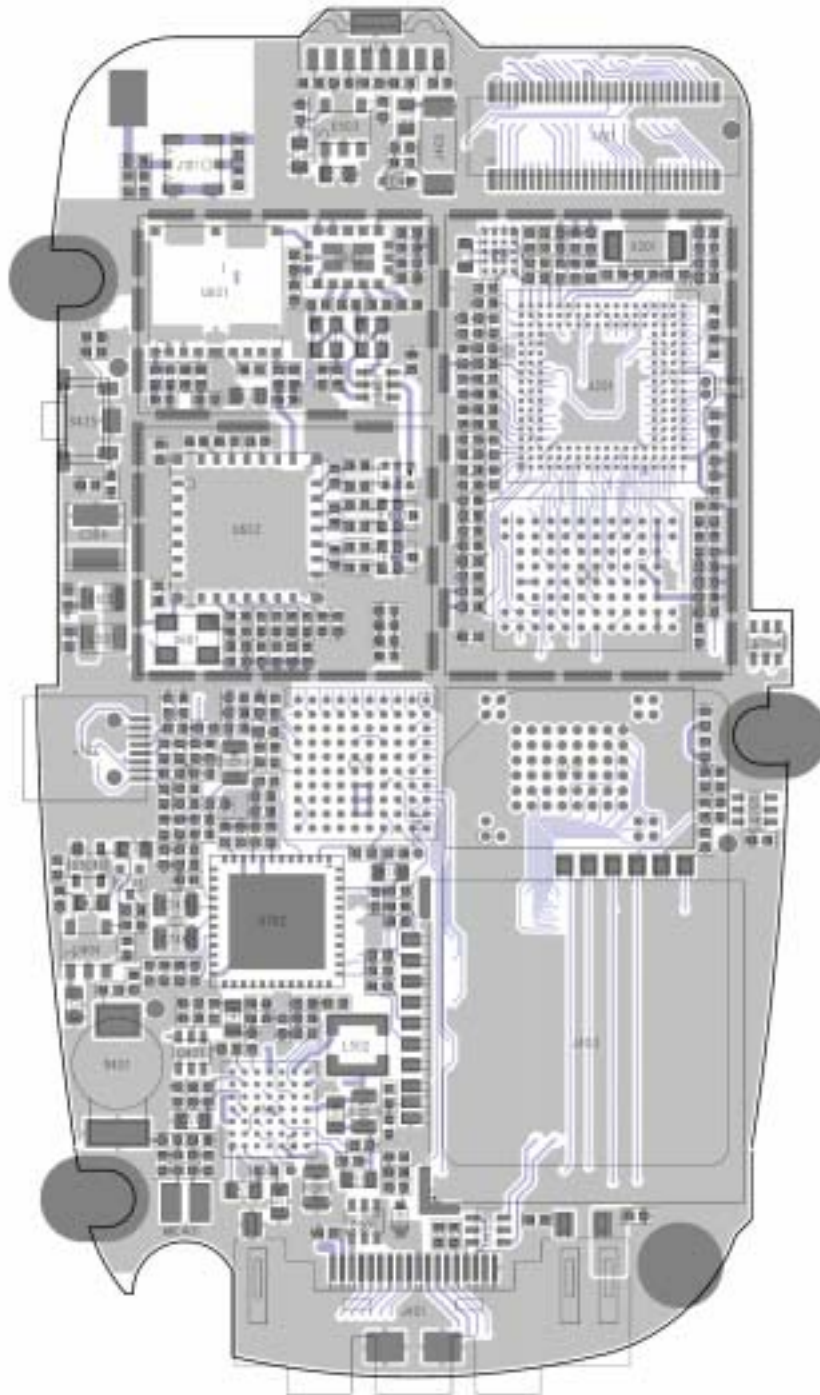
<Figure 5.5> BASEBAND Area
