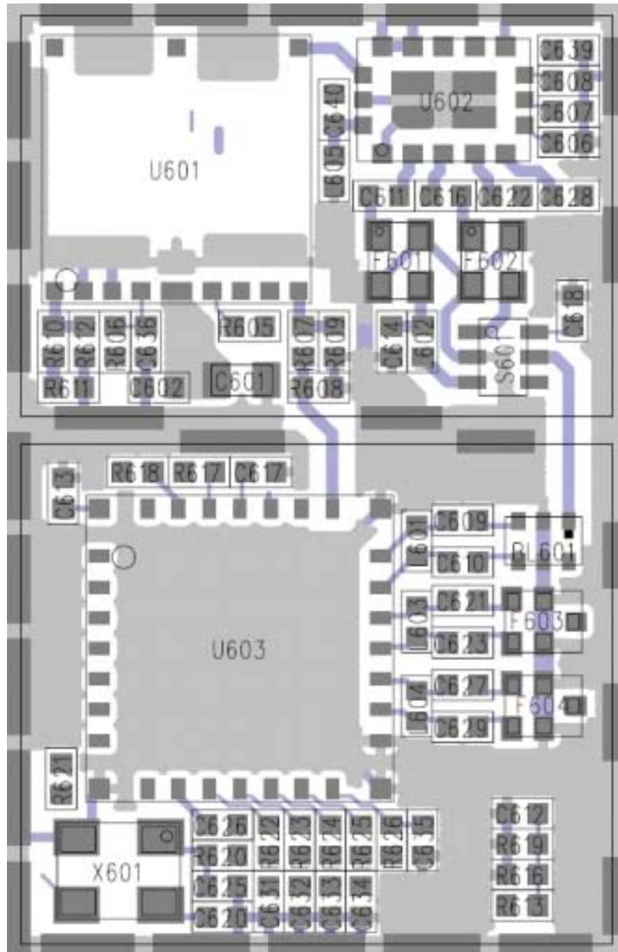
<Figure 5.4> RF Area
