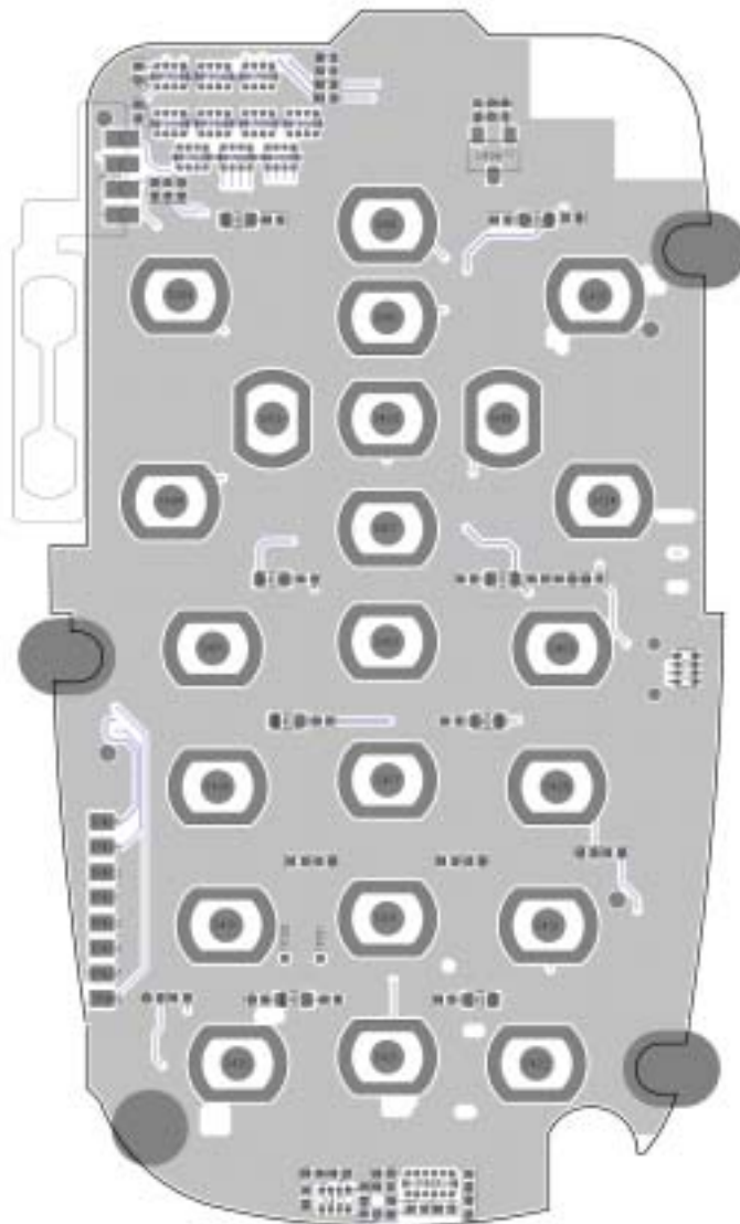
<Figure 5.1> Top View
