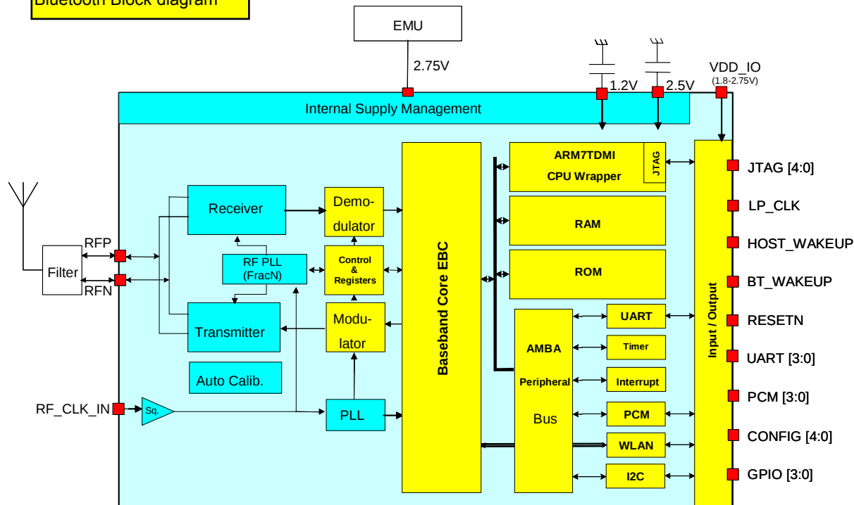
Bluetooth Block diagram
