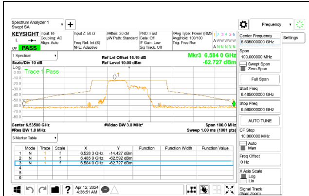
LOW CHANNEL Antenna 1
