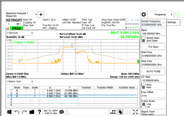
LOW CHANNEL Antenna 3
