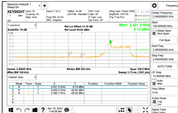
LOW CHANNEL 4 BANDEDGE Antenna 1
