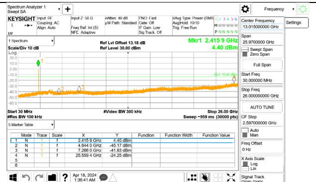
OUT-OF-BAND LOW CHANNEL 3 Antenna 1
