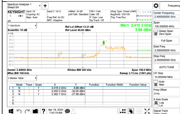
LOW CHANNEL 3 BANDEDGE Antenna 3
