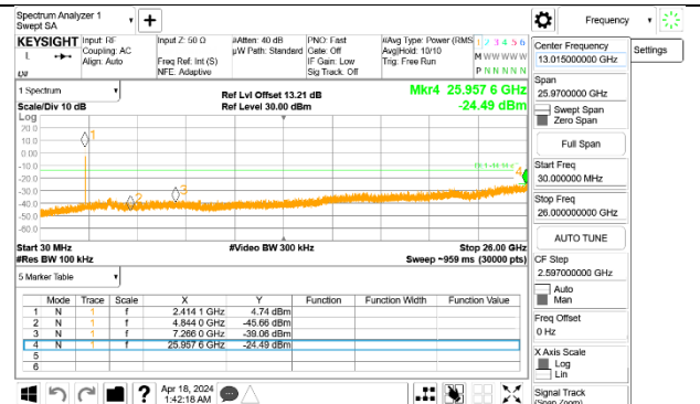
OUT-OF-BAND LOW CHANNEL 3 Antenna 3
