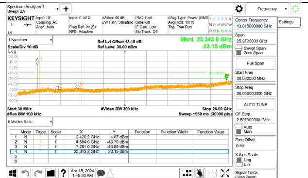
OUT-OF-BAND LOW CHANNEL 4 Antenna 1
