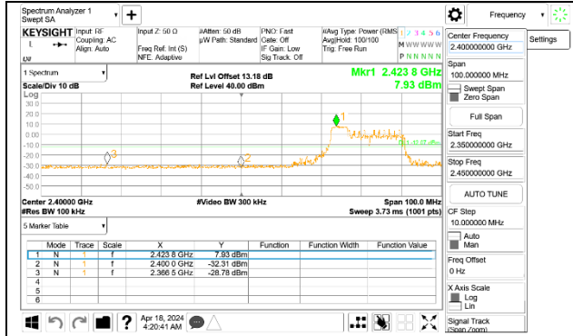
LOW CHANNEL 5 BANDEDGE Antenna 1
