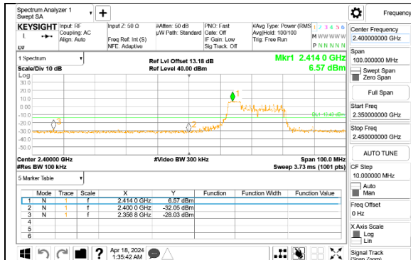
LOW CHANNEL 3 BANDEDGE Antenna 1
