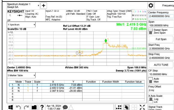
LOW CHANNEL 4 BANDEDGE Antenna 3
