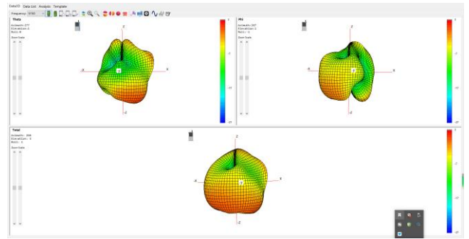
5150MHZ 3D
