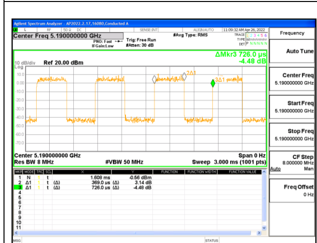
802.11ax HE40 OFDMA, RU size 484T MODE
