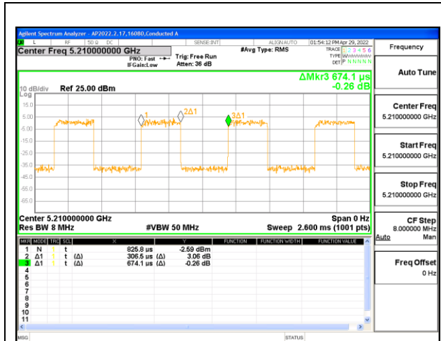
802.11ax HE80 OFDMA, OFDMA MODE: SU
