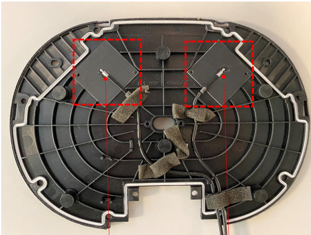
WiFi Antenna ANT2
