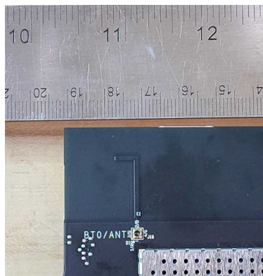
BT Antenna (close-up, 180° from above picture)
