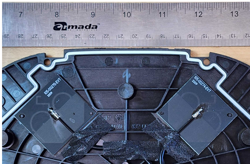
WiFi Antenna ANT2 and ANT3 (close-up)
