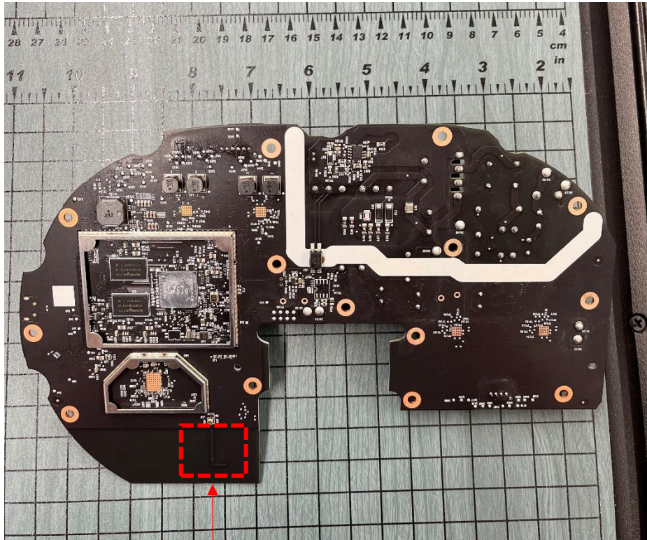
Bluetooth Antenna
