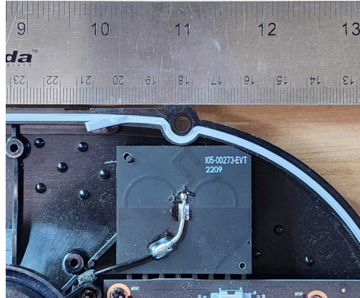
WiFi Antenna ANT4 (close-up)
