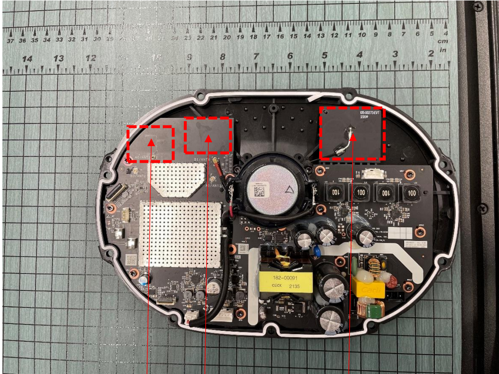
WiFi Antenna ANT1
