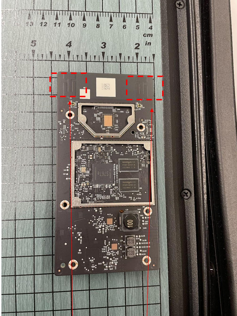
WiFi Antenna Chain 1 - ANT4
