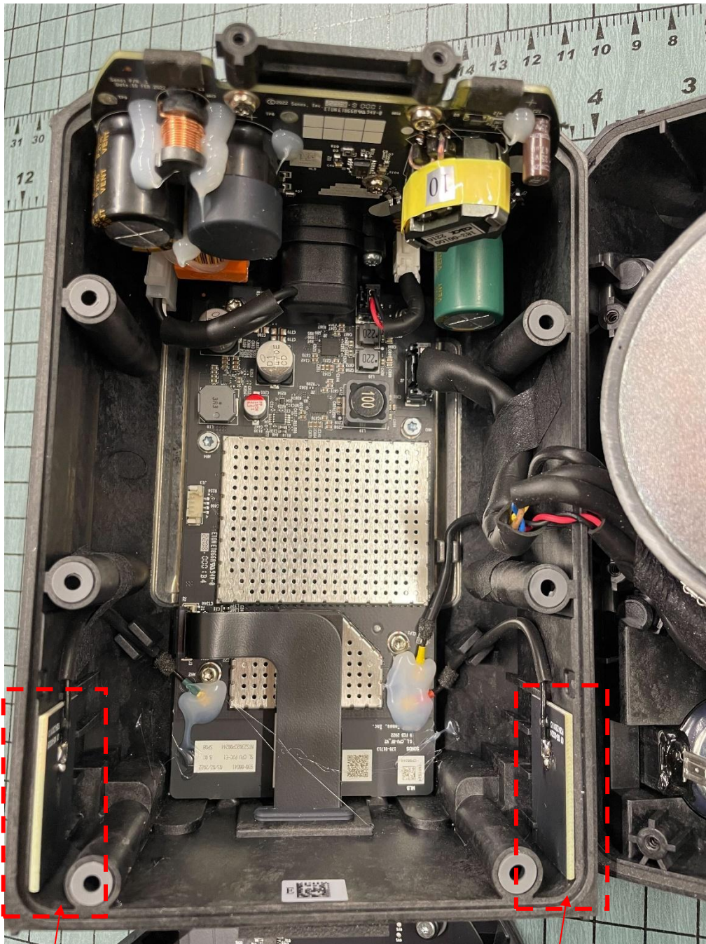
WiFi Antenna Chain 0 - ANT2
