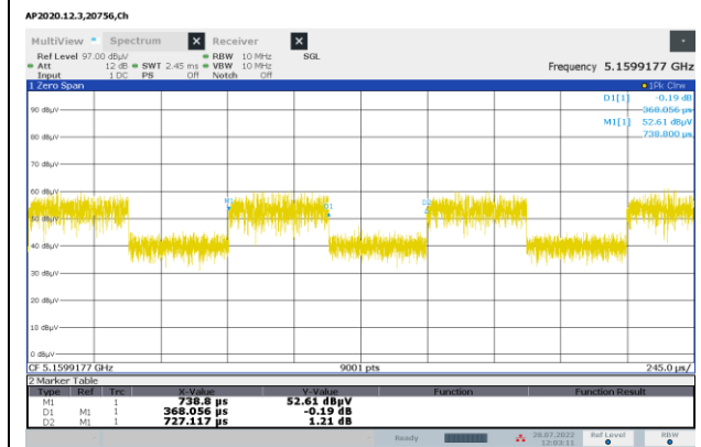
802.11ax HE40 OFDMA, RU size 484T MODE
