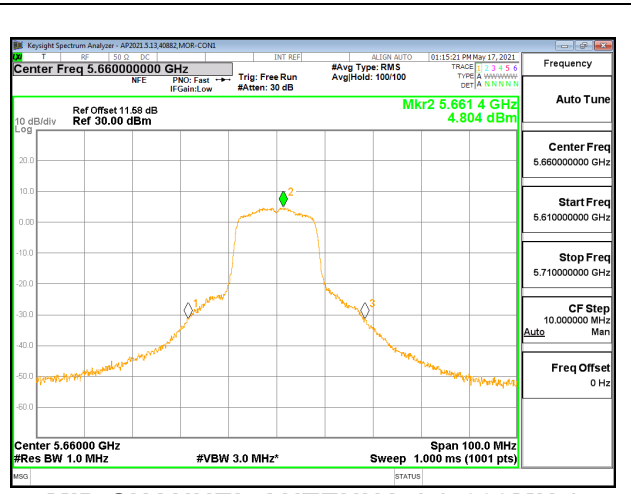
MID CHANNEL ANTENNA 1 (5660MHz)
