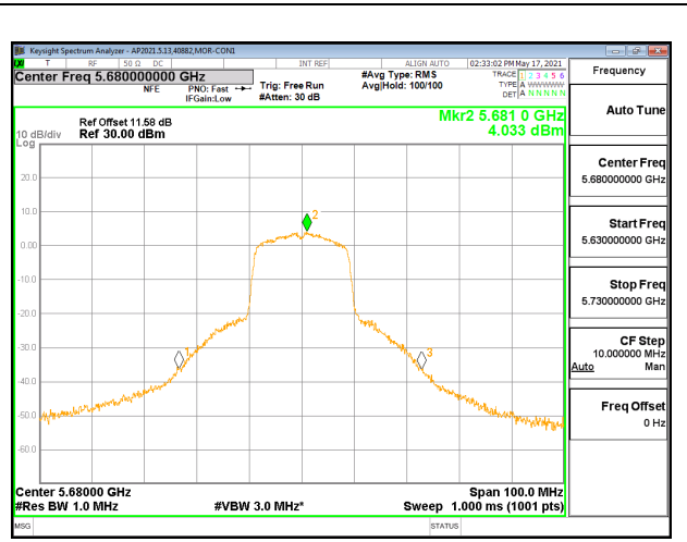
HIGH CHANNEL (5680MHz) ANTENNA 1
