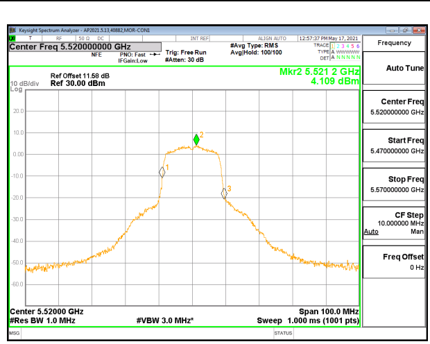
LOW CHANNEL (5520 MHz) ANTENNA 1
