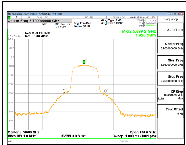
HIGH CHANNEL (5700MHz) ANTENNA 0
