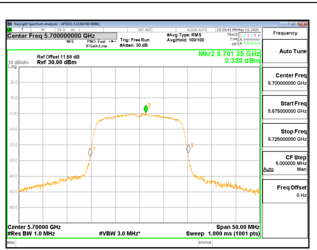
HIGH CHANNEL (5700MHz) ANTENNA 1
