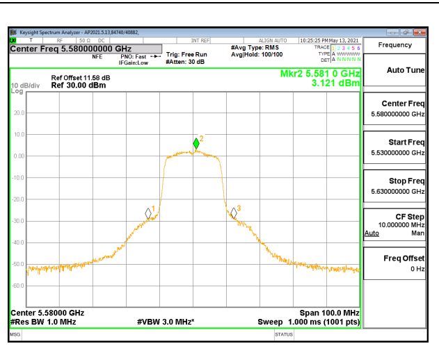
MID CHANNEL (5580MHz) ANTENNA 1
