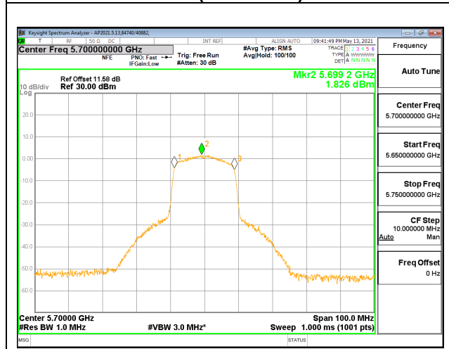
HIGH CHANNEL ANTENNA 0
