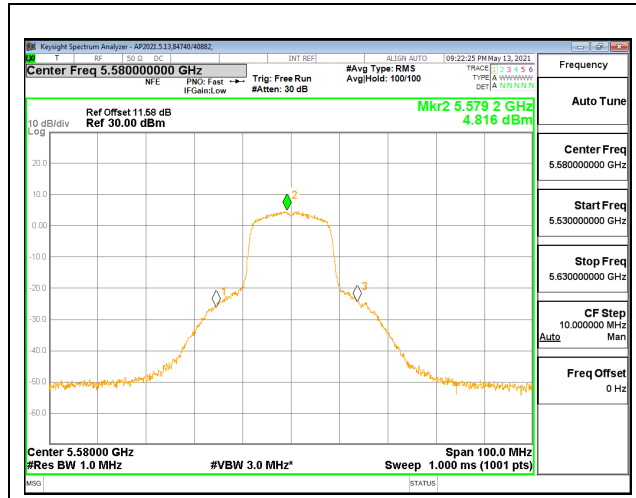
MID CHANNEL (5580MHz) ANTENNA 0
