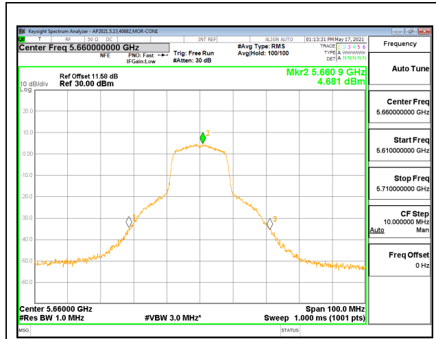
MID CHANNEL ANTENNA 0 (5660MHz)
