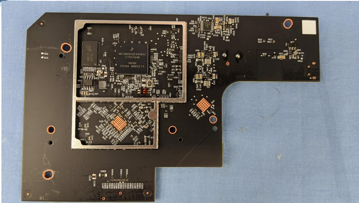
RF Board Back Shields Removed
