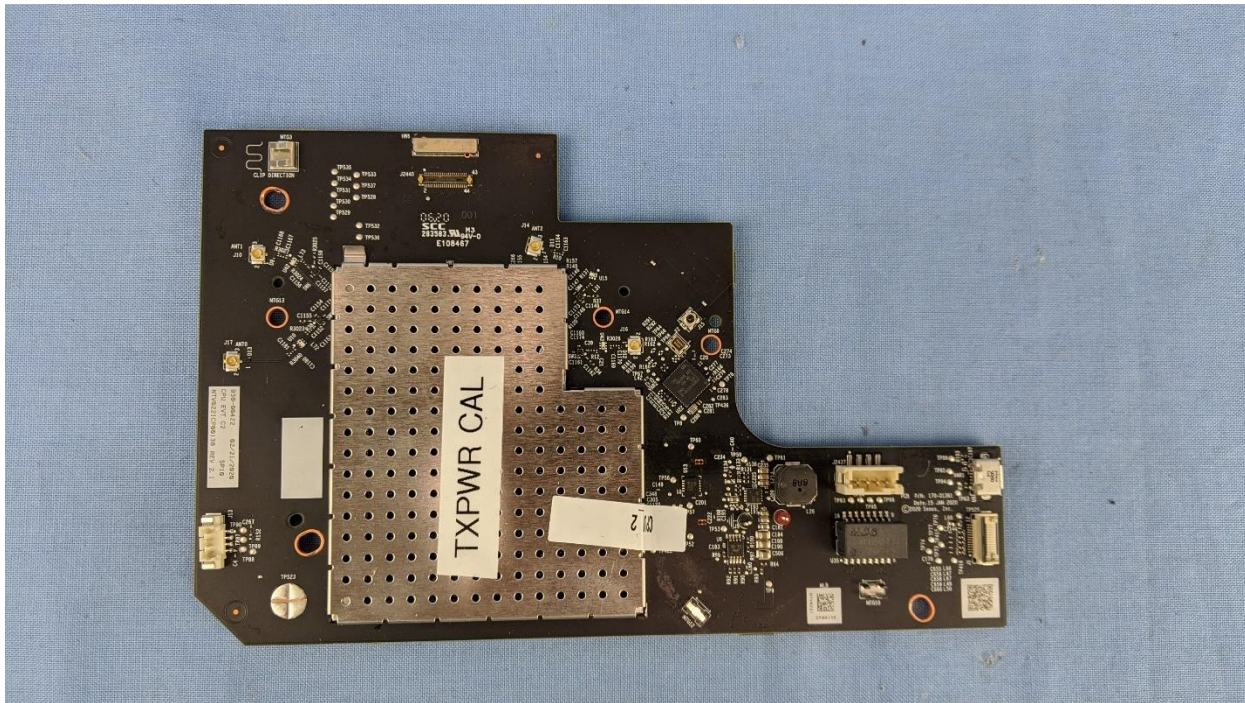
RF Board Front
