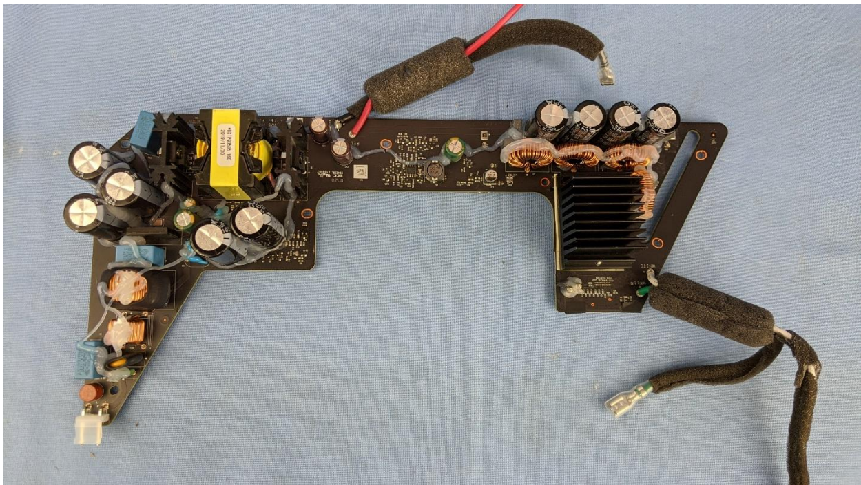
Power Board Front
