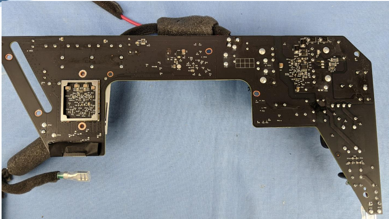
Power Board Back Shields Removed
