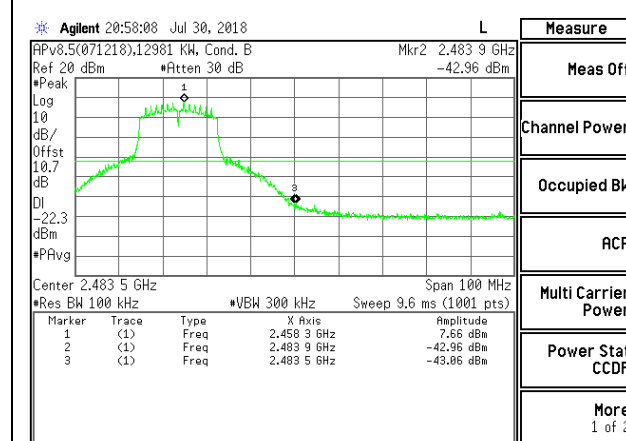
HIGH CHANNEL 10 BANDEDGE CHAIN 1
