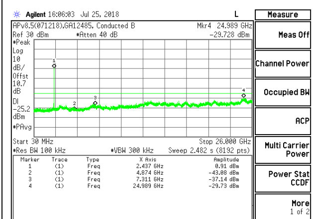
OUT-OF-BAND MID CHANNEL CHAIN 1
