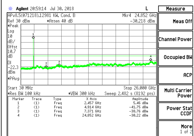
OUT-OF-BAND HIGH CHANNEL 10 CHAIN 1
