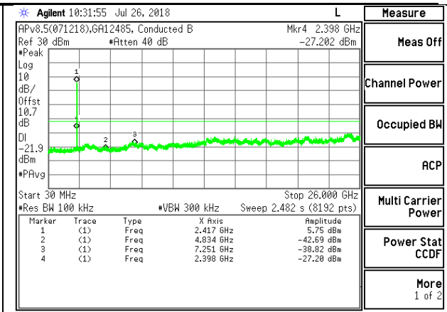
OUT-OF-BAND LOW CHANNEL 2 CHAIN 1
