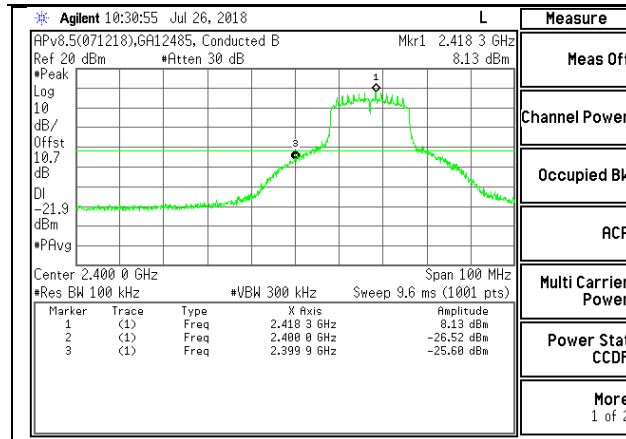
LOW CHANNEL 2 BANDEDGE CHAIN 1
