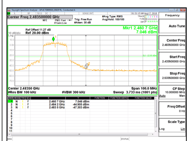
HIGH CHANNEL 11 BANDEDGE CHAIN 2
