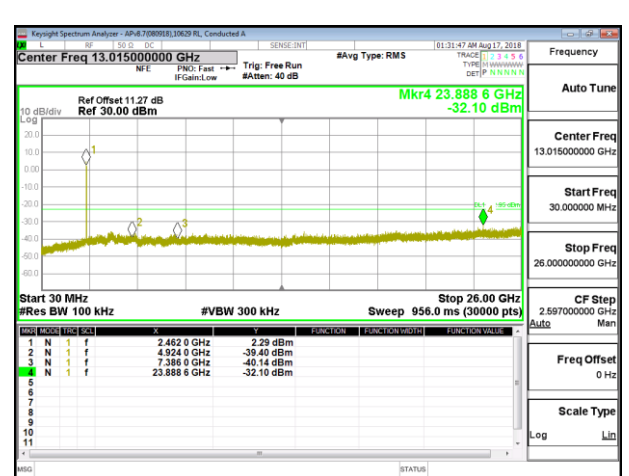
OUT-OF-BAND HIGH CHANNEL 11 CHAIN 2
