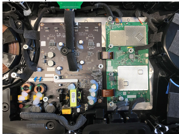
Detail of PCBA in product
