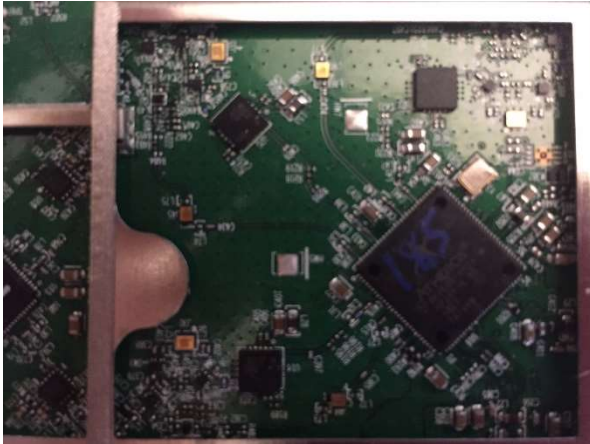
Original Layout
