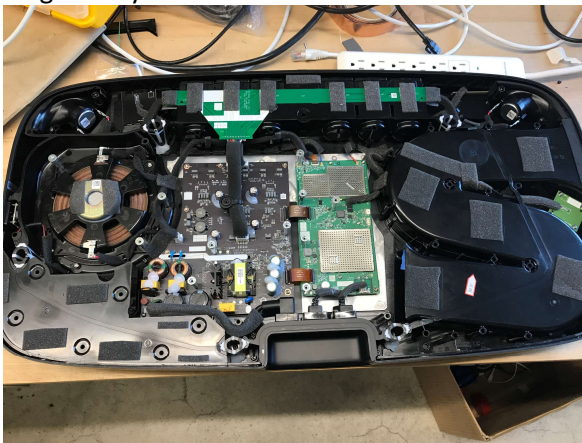
PCBA mounting position in Product
