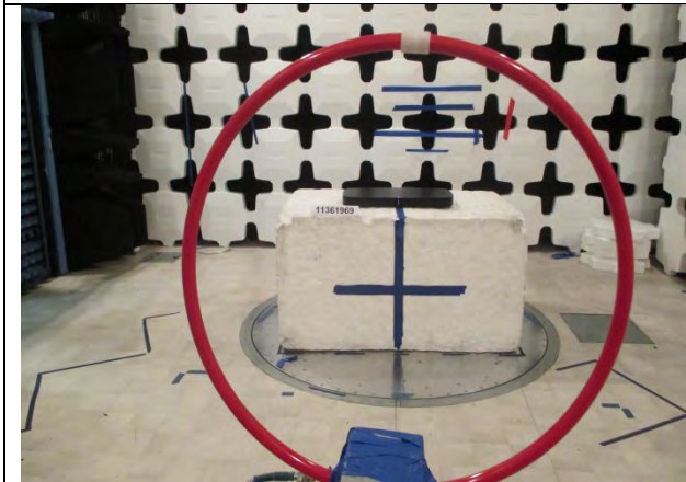
RADIATED FRONT PHOTO (BELOW 30 MHz)
