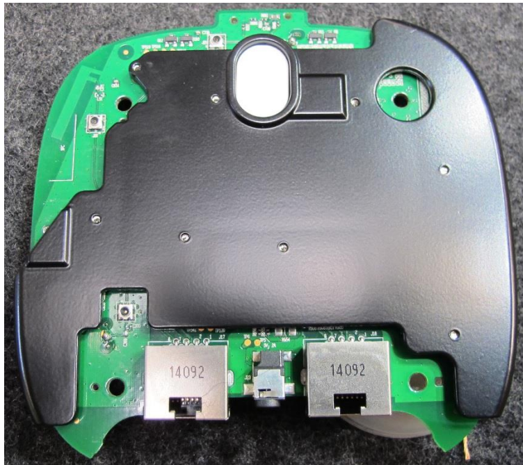
Main PCB bottom with shield
