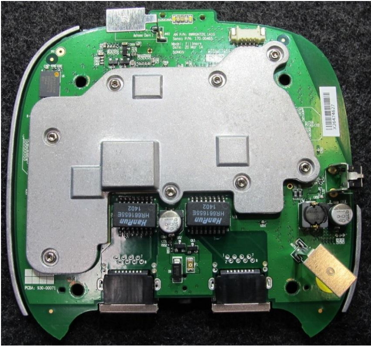
Main PCB top
