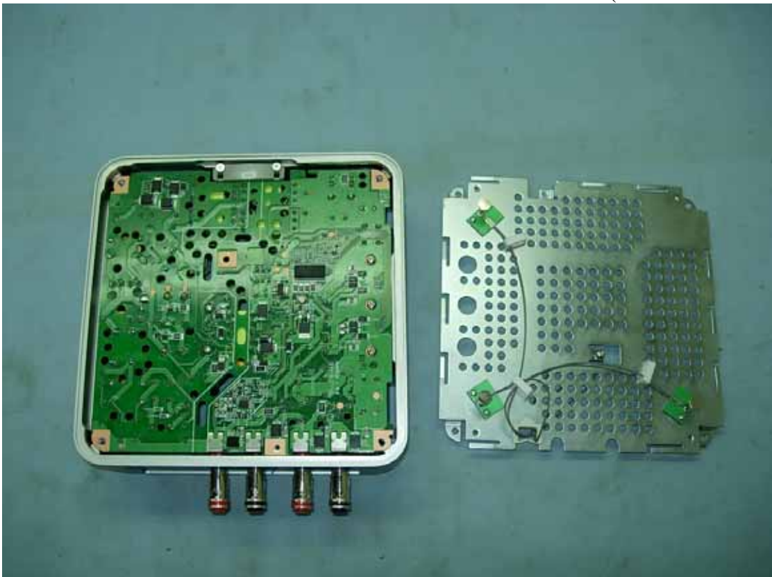
Figure 14 Internal View (Removed Shield Cover)
