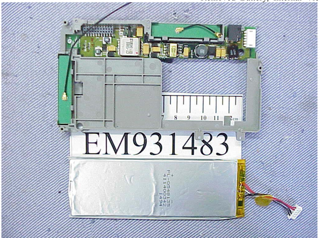
Figure 4 Removed Battery, Internal View
