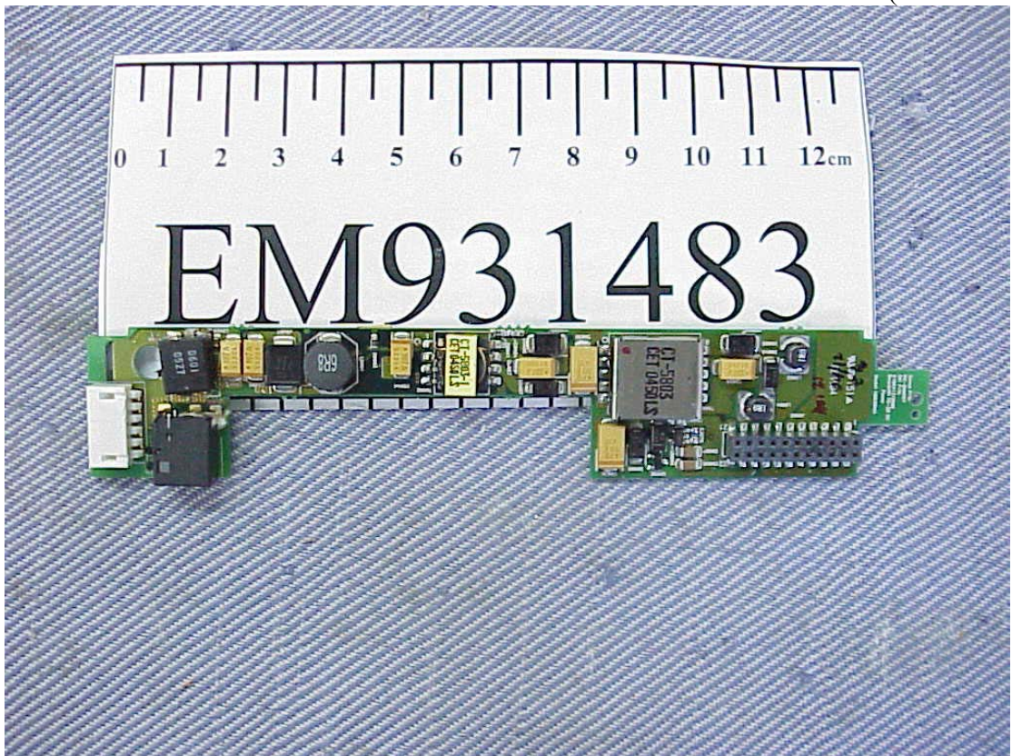
Figure 8 RX Board (Front Side)
