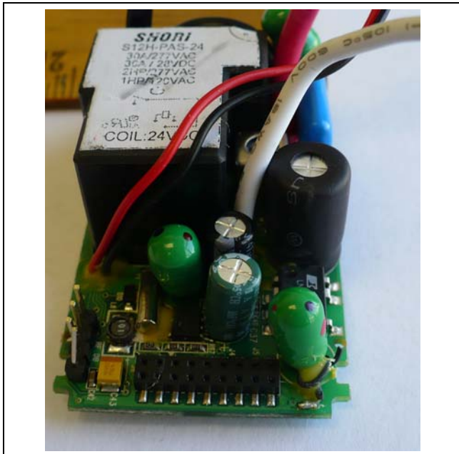
Logic-Power PCB Side View
