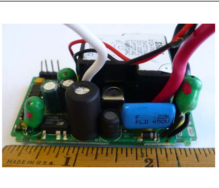
Logic-Power PCB Side View
