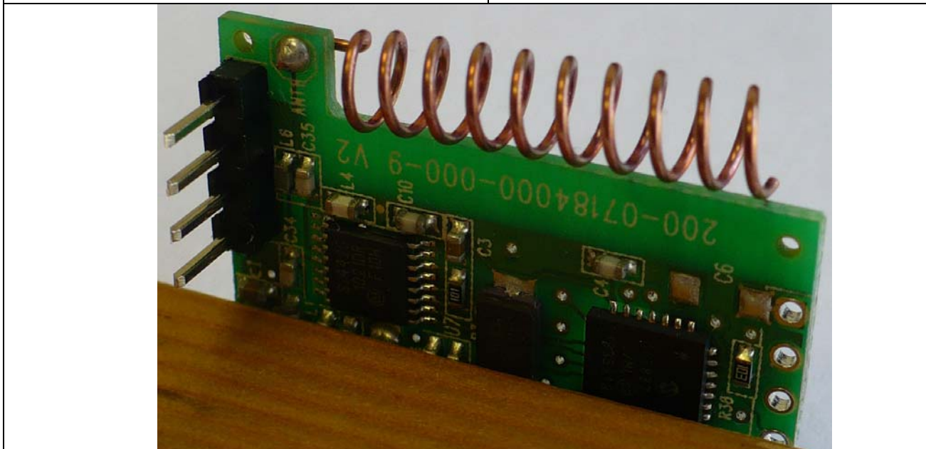
RF Daughter PCB - Side View & Antenna Close-up
