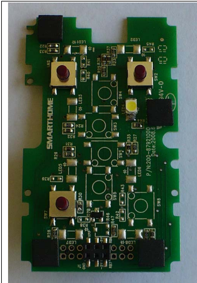
Switch-LED PCB Top View
