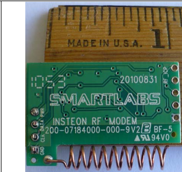
RF Daughter PCB Top View
