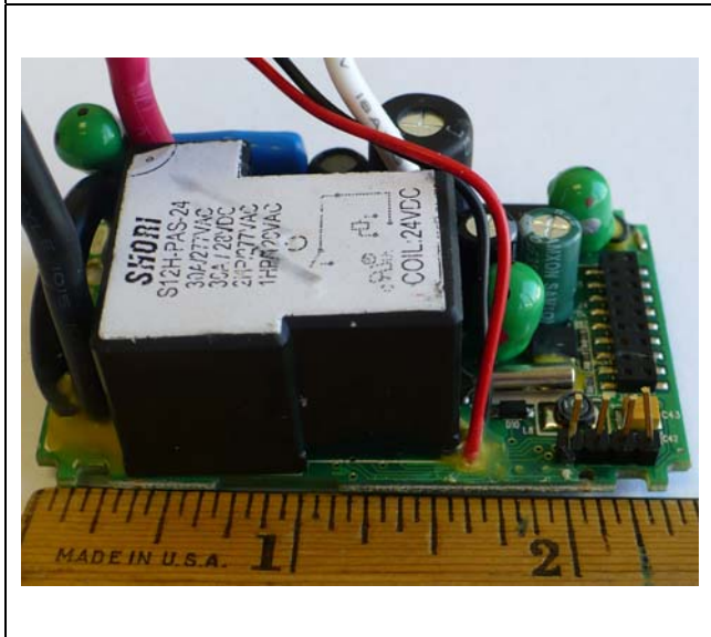
Logic-Power PCB Side View
