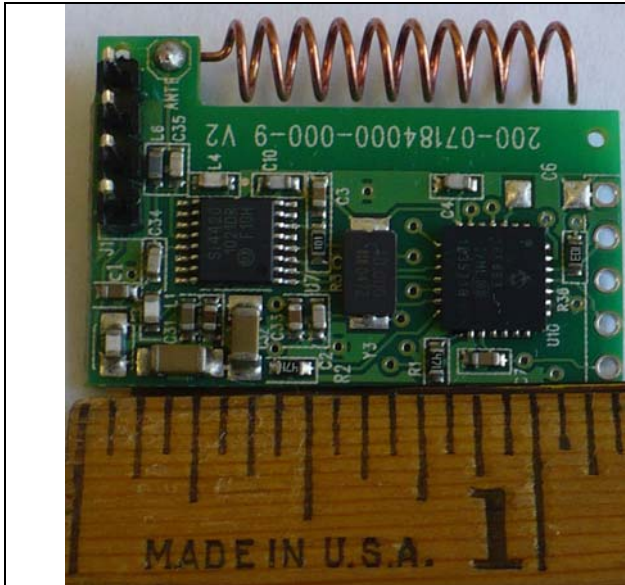
RF Daughter PCB Top View
