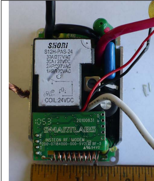
Back Case Removed Top View
