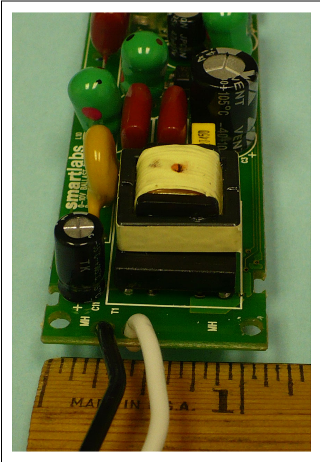
Main PCB Top Power Input Side View
