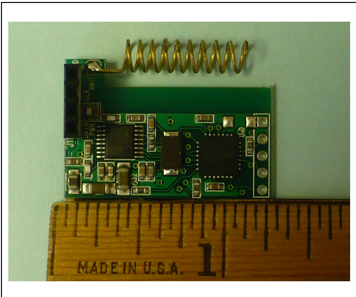
RF Daughter PCB Top View
