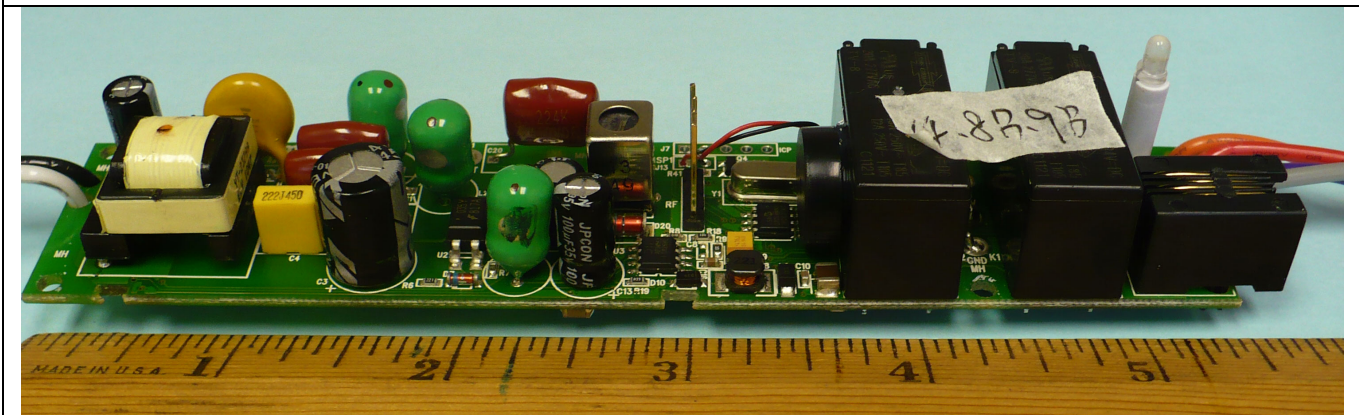
Main PCB Top Side 2 View
