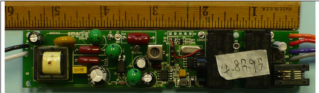
Main PCB Top View
