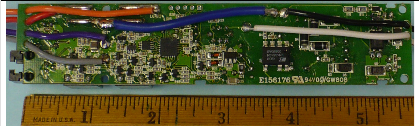
Main PCB Bottom View
