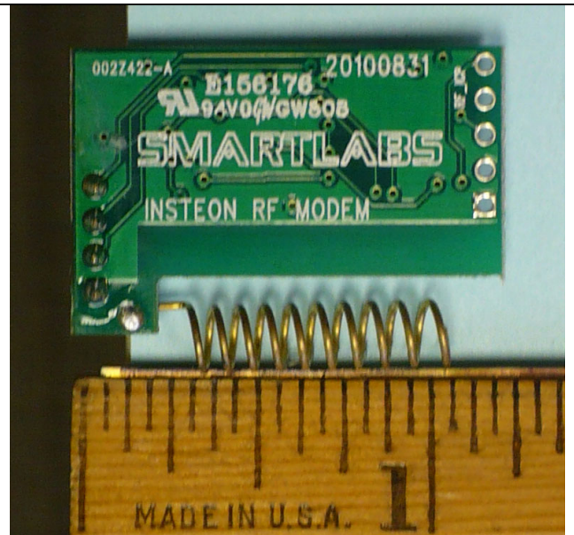
RF Daughter PCB Top View
