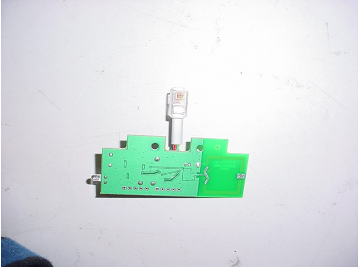
PCB – Solder View
