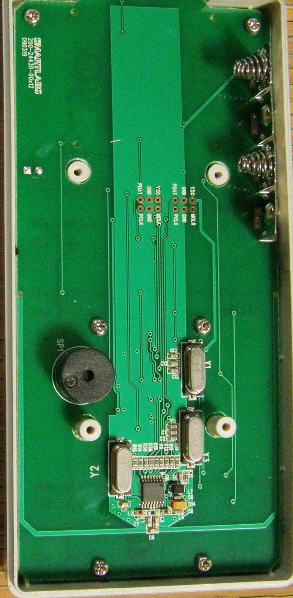
PCB IN FRONT PANEL & INSIDE VIEW BACK PANEL
