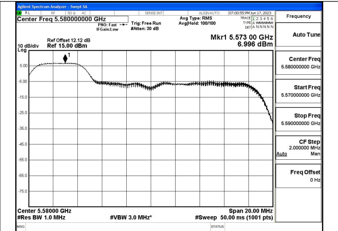
Mode:802.11ax HE20 Tone:52T Frequency:5580MHz Ant:Chain0
