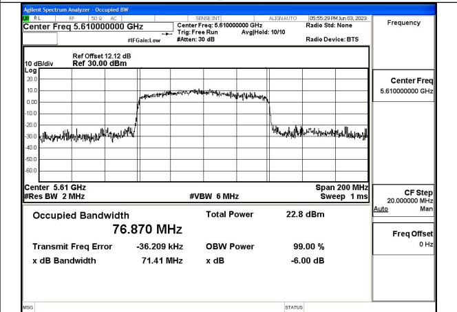
Mode:802.11ax HE80 Frequency:5610MHz Ant:Chain1
