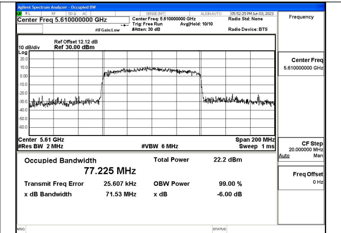
Mode:802.11ax HE80 Frequency:5610MHz Ant:Chain0
