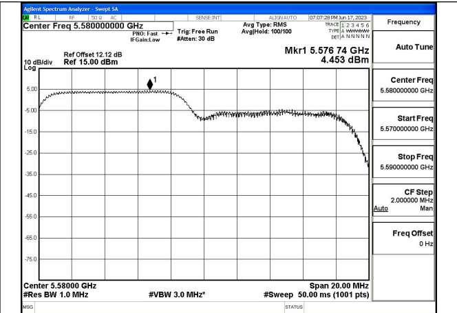
Mode:802.11ax HE20 Tone:106T Frequency:5580MHz Ant:Chain0
