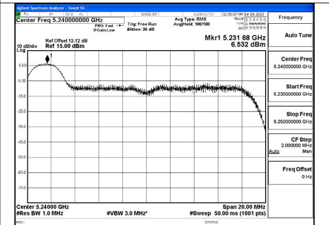
Mode:802.11ax HE20 Tone:26T Frequency:5240MHz Ant:Chain1
