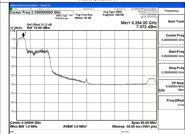
Mode:802.11ax HE80 Tone:52T Frequency:5290MHz Ant:Chain1
