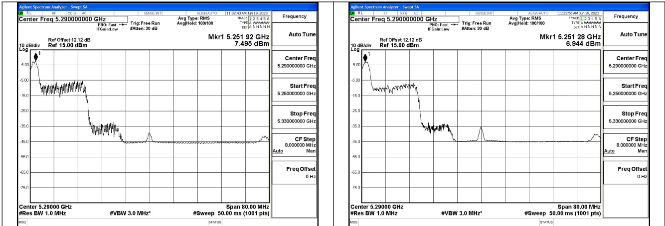
Mode:802.11ax HE80 Tone:26T Frequency:5290MHz Ant:Chain0
