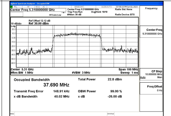
Mode:802.11ax HE40 Frequency:5310MHz Ant:Chain1
