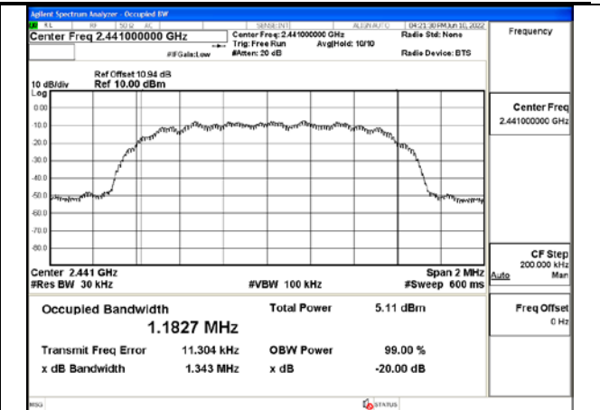
Test Mode:π/4QPSK(2DH5) MHz
