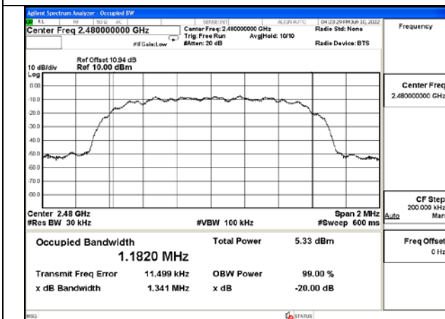
Test Mode:π/4DQPSK(2DH5) MHz
