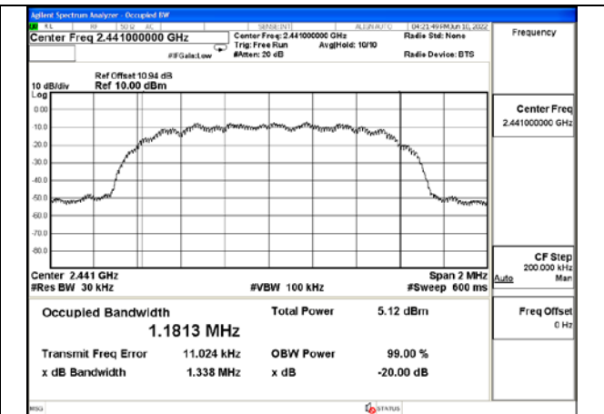
Test Mode:π/4DQPSK(2DH5) MHz
