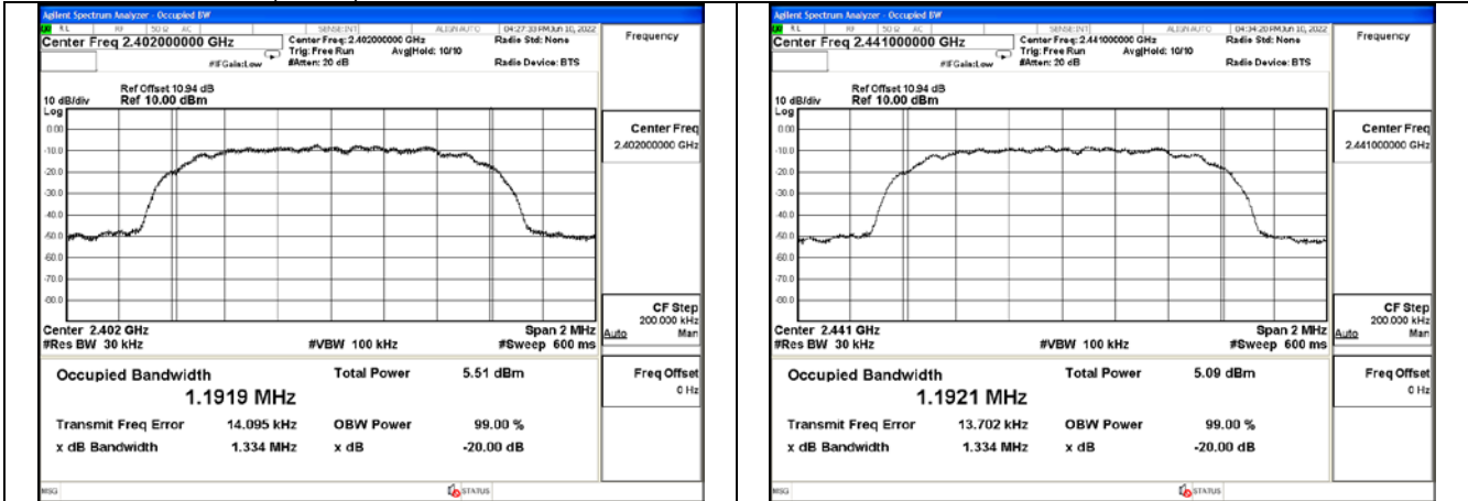
Test Mode:8DPSK(3DH5) MHz
