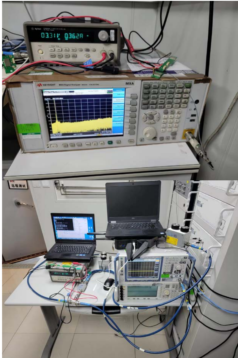
RF Conducted Test setup (BT/WIFI)
