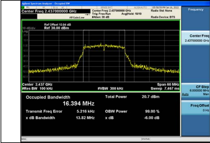
Test Mode:802.11g 2437MHz Chain1
