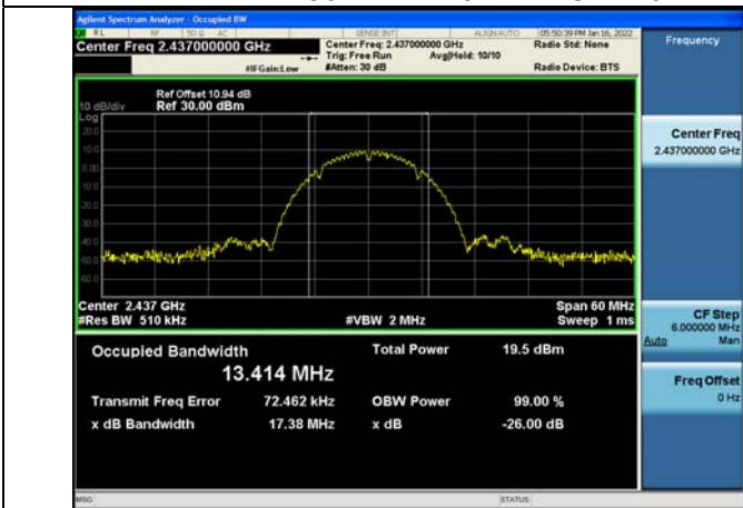
Test Mode:802.11b 2437MHz Chain1
