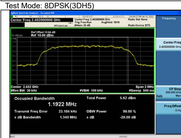
Test Mode:8DPSK(3DH5) MHz
