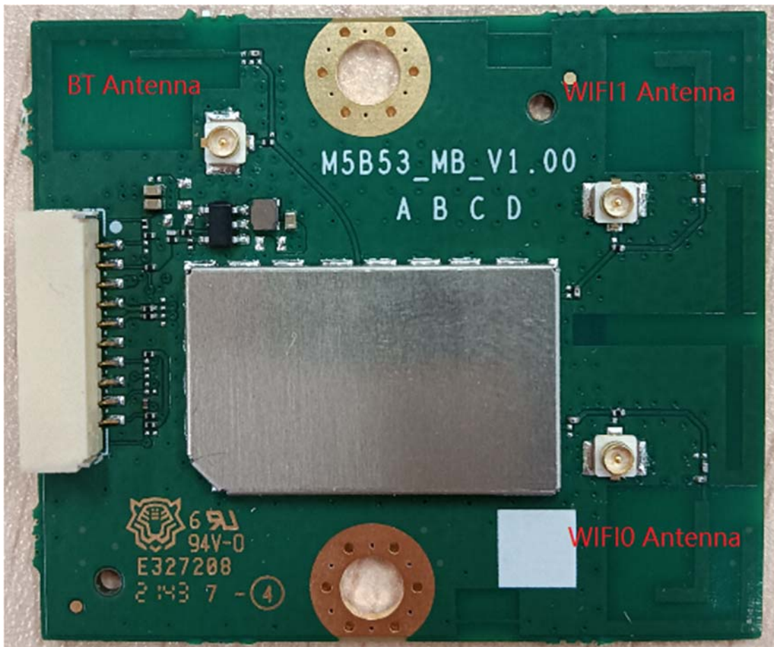
Antenna Location
