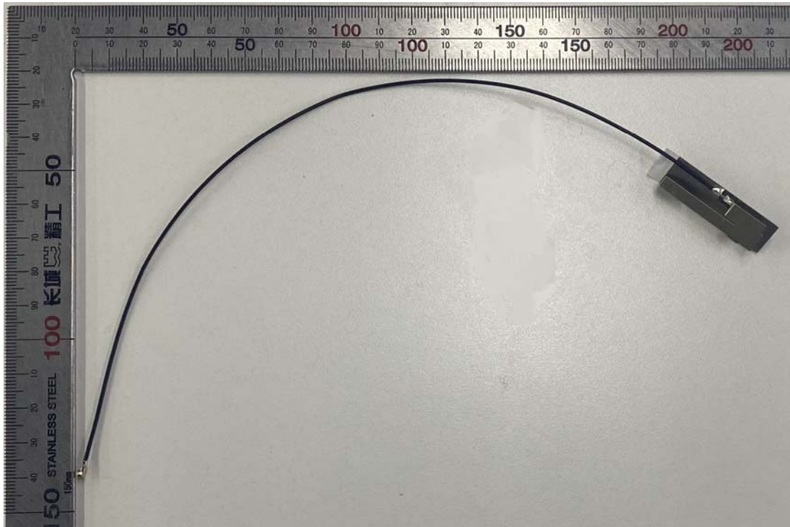
External Antenna
