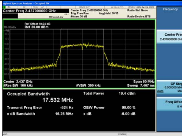
Test Mode:802.11n HT20 2437MHz Chain1
