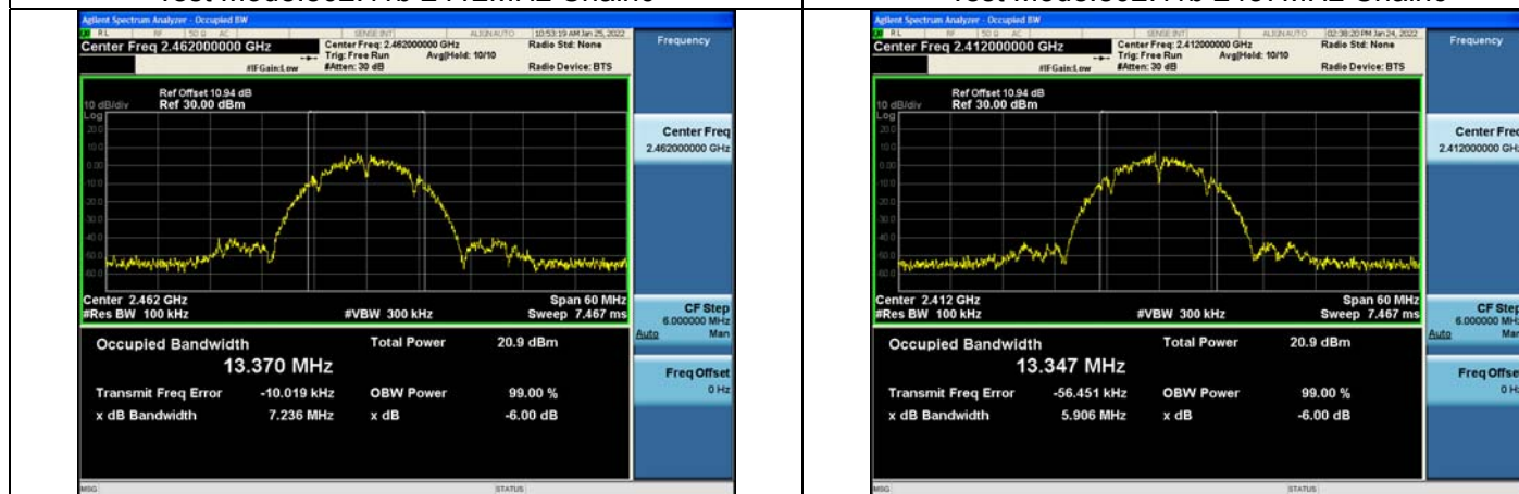
Test Mode:802.11b 2462MHz Chain0
