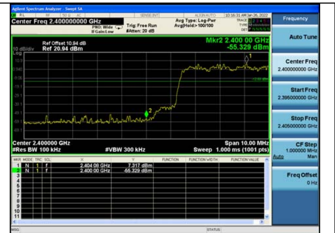
CH0(Hopping on)
