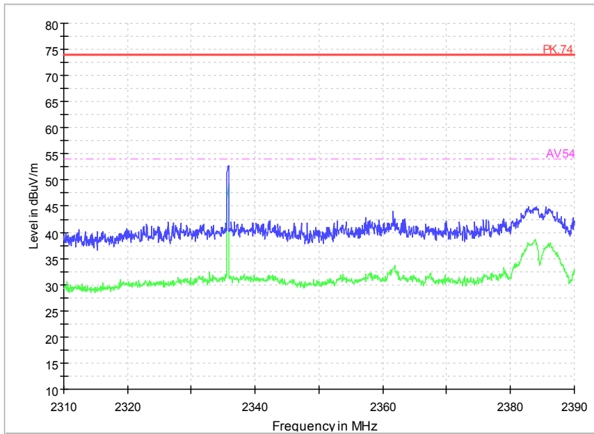
Carrier frequency (MHz): 2412 Channel No.:1 Test Mode: 802.11 n(HT20) Polarity:Vertical
