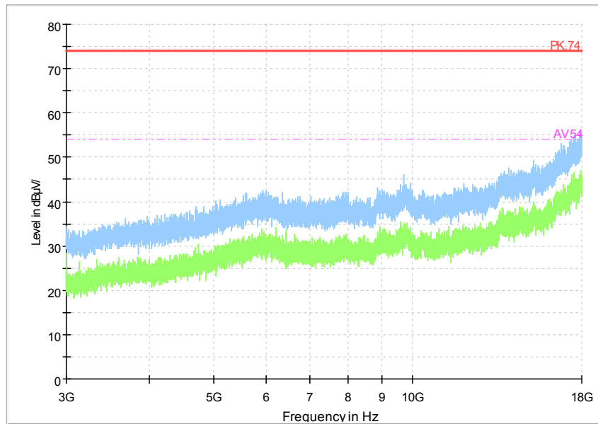
Frequency Range: 3GHz -18GHz Detector: Av mode and PK mode Modulation type: 802.11n(HT40)
