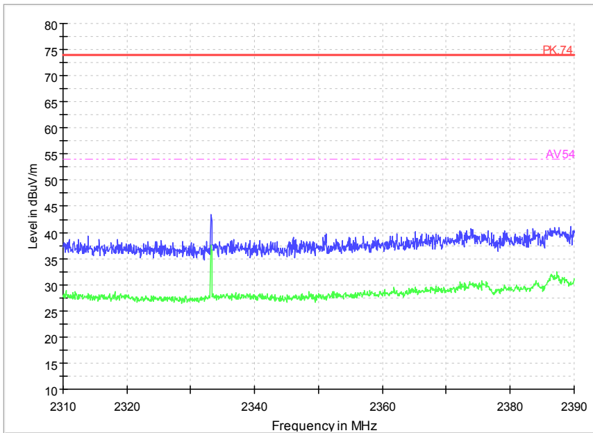
Carrier frequency (MHz): 2412 Channel No.:1 Test Mode: 802.11 n(HT20) Polarity: Horizontal
