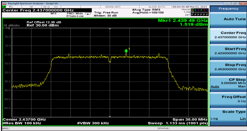
11N20SISO_Ant1_2437_0~Reference
