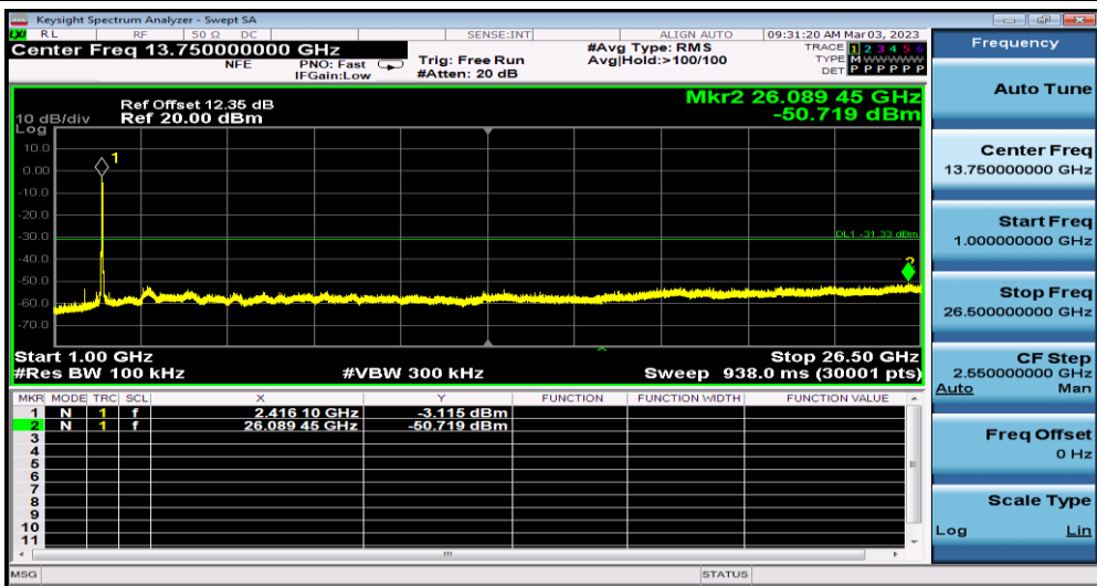
11N40SISO_Ant1_2422_1000~26500
