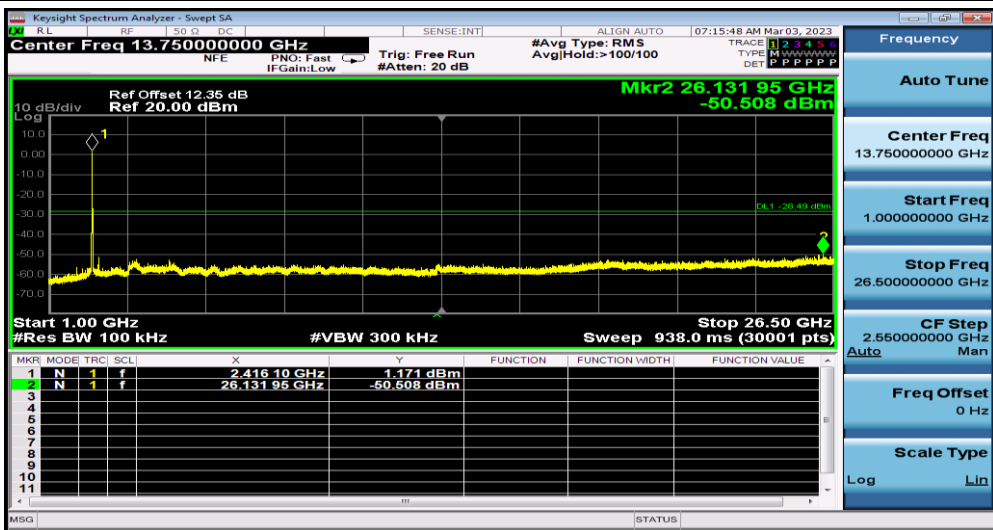
11N20SISO_Ant1_2412_1000~26500
