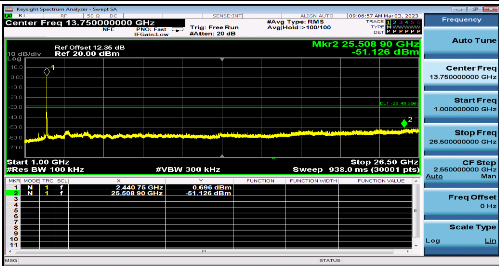
11N20SISO_Ant1_2437_1000~26500
