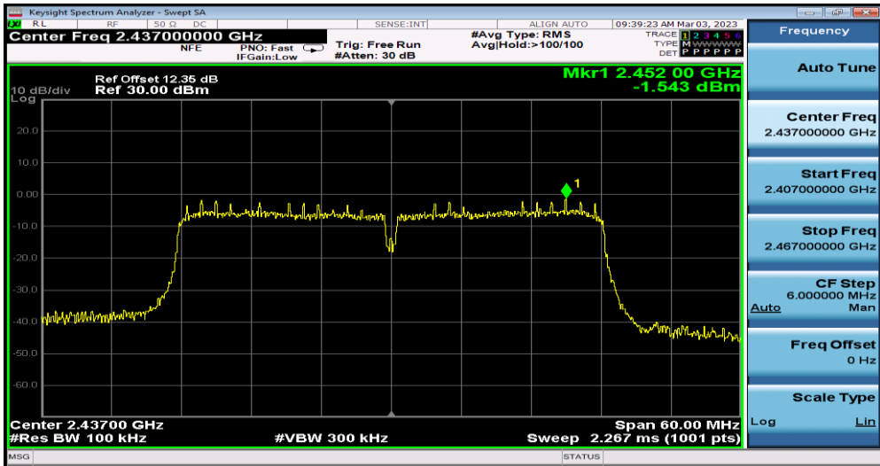
11N40SISO_Ant1_2437_0~Reference
