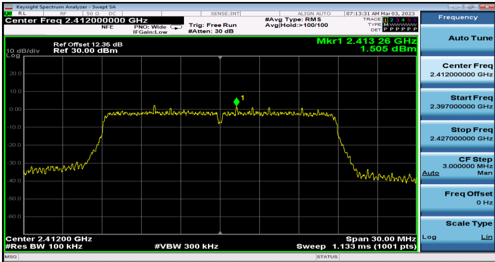
11N20SISO_Ant1_2412_0~Reference
