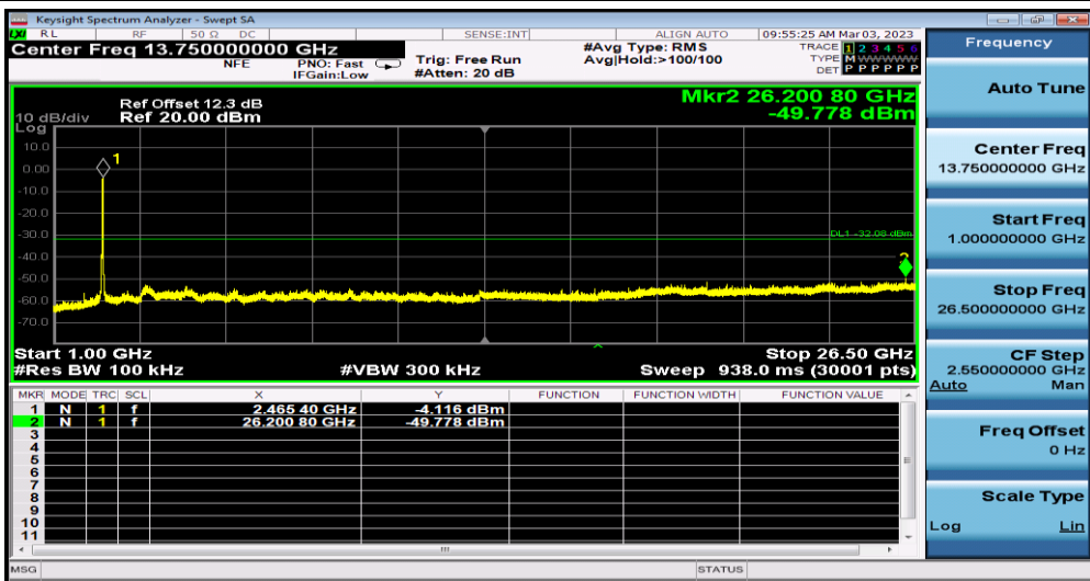
11N40SISO_Ant1_2452_1000~26500
