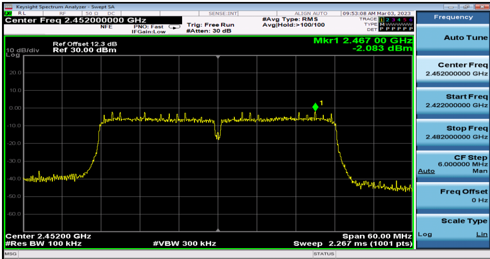
11N40SISO_Ant1_2452_0~Reference
