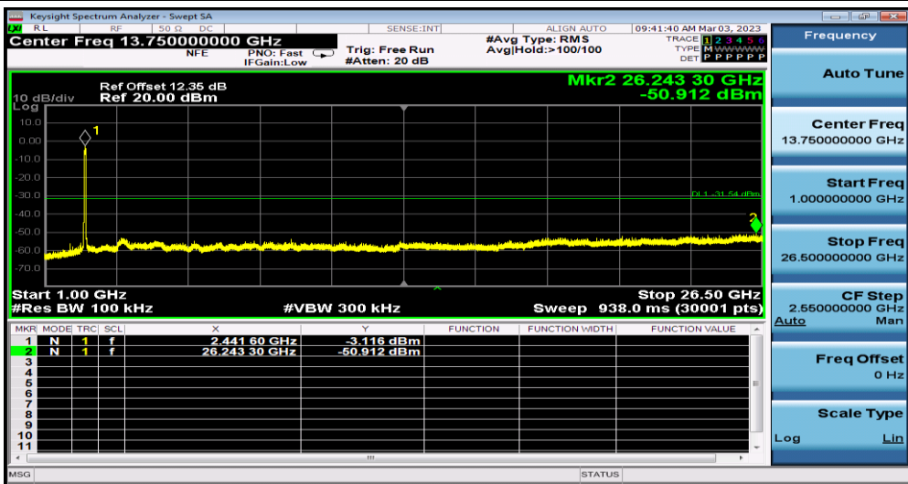
11N40SISO_Ant1_2437_1000~26500
