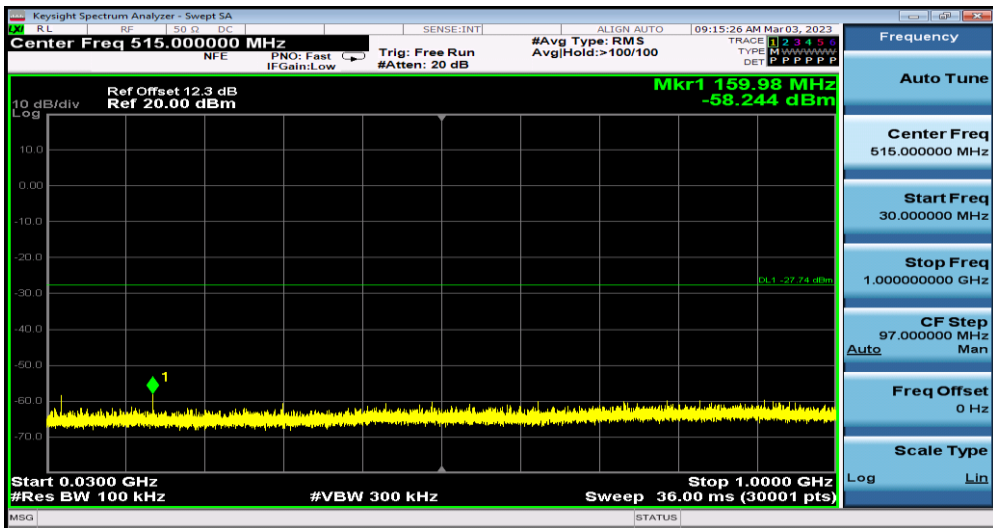
11N20SISO_Ant1_2462_30~1000
