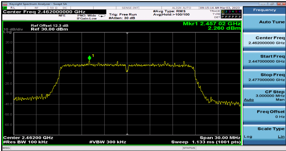
11N20SISO_Ant1_2462_0~Reference
