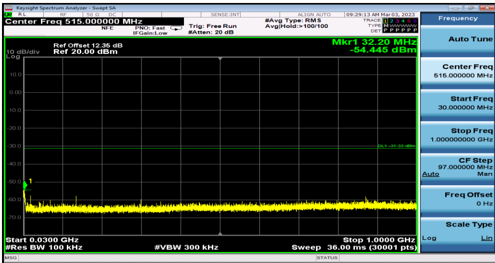
11N40SISO_Ant1_2422_30~1000
