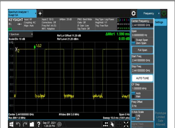
Modulation: GFSK DH3 2441MHz
