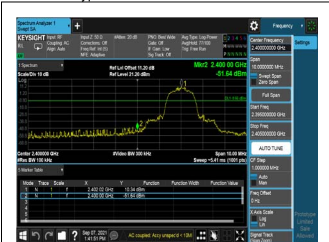
CH0(Hopping off)
