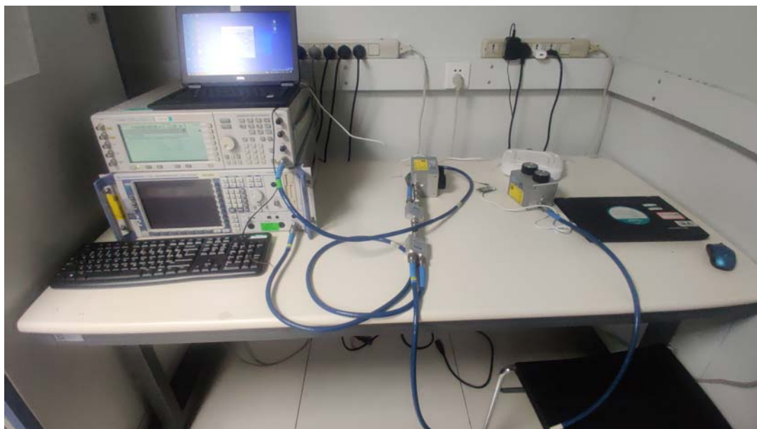
Dynamic Frequency Selection Test setup
