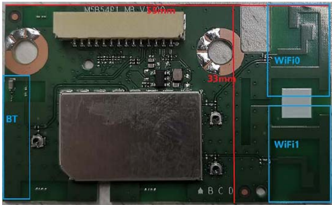
Ant location
