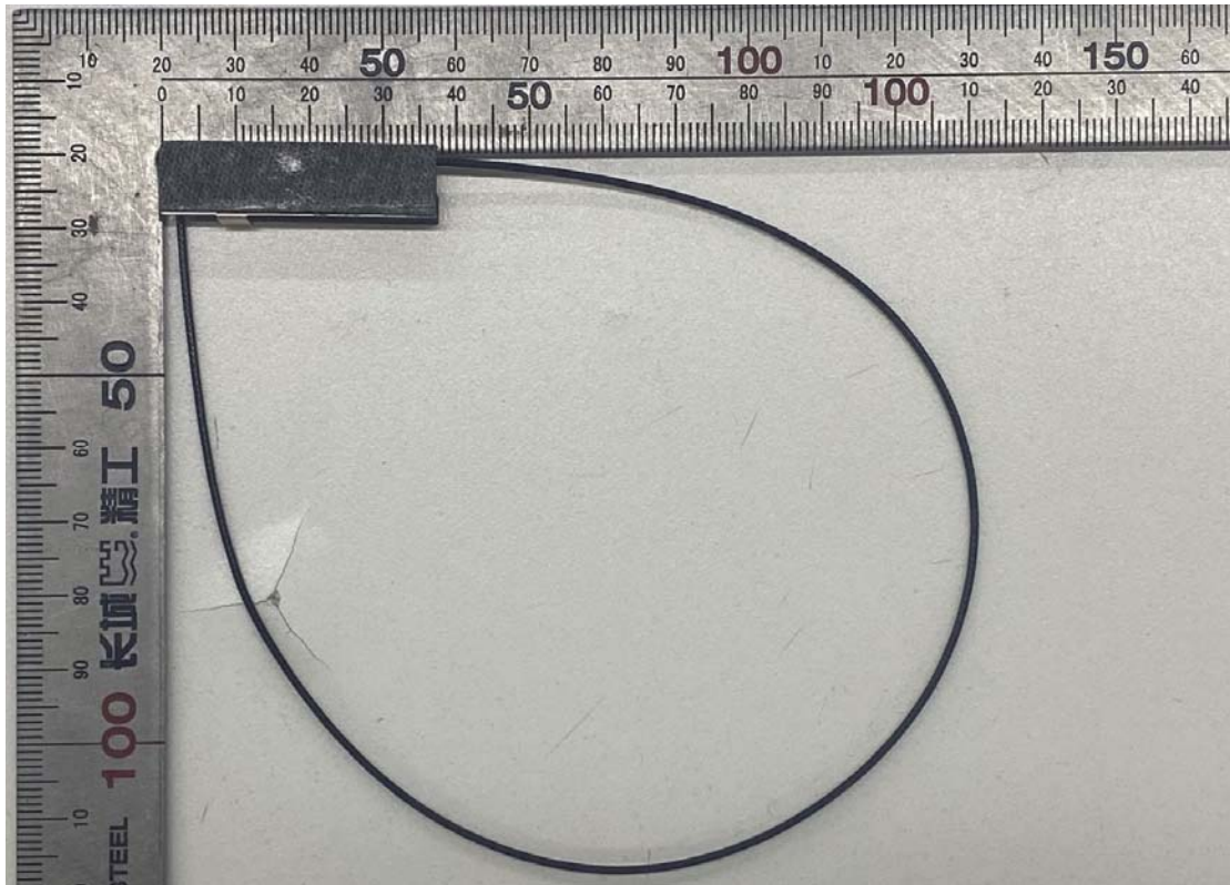
External IPEX Antenna
