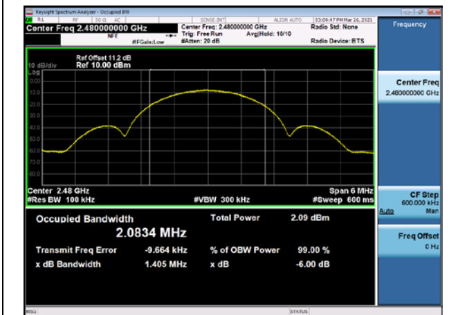
Modulation: 2Mbps 2480MHz
