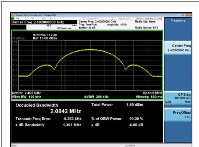
Modulation: 2Mbps 2402MHz
