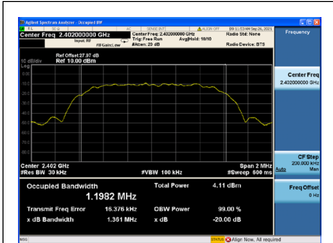
Modulation: 8DPSK 2402MHz
