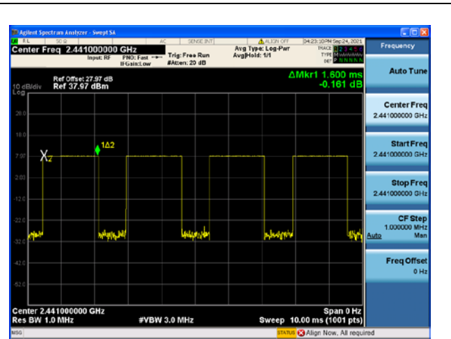
Modulation: GFSK DH3 2441MHz
