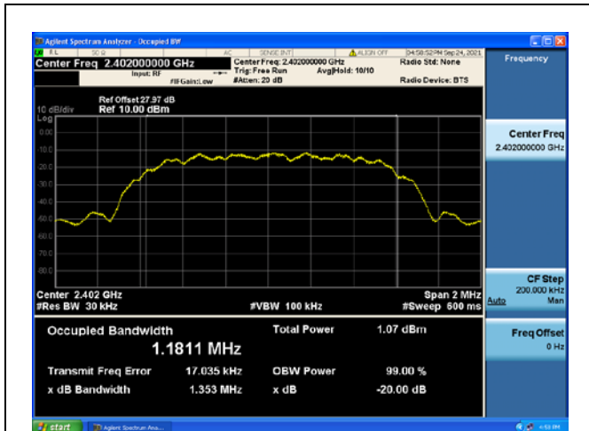
Modulation: \pi/4 DQPSK 2402MHz
