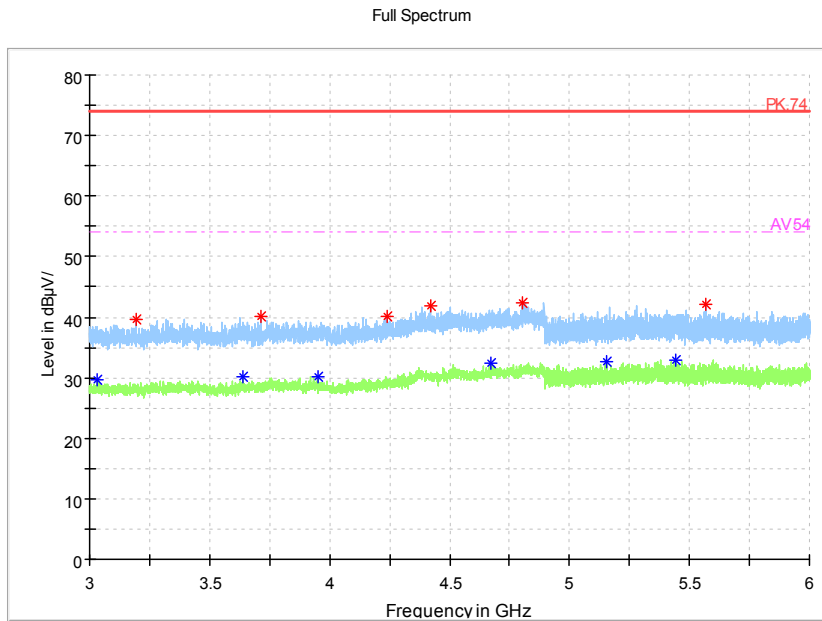
Frequency Range: 3GHz -6GHz Detector: Av mode and PK mode Modulation type: 802.11n(HT40 MIMO)
