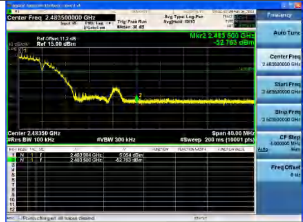
Test Mode:802.11b Chain1 CH11
